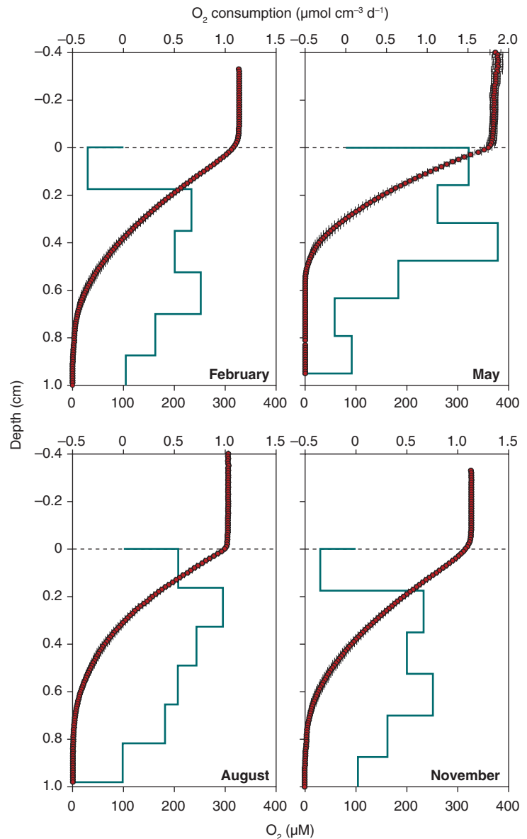
Figure 5.20 Vertical concentration profiles of oxygen (closed dots) and modelled consumption rates (solid line) from microelectrode profiles with sediment depth for each of the four sampling periods. Error bars represent standard error of the mean.
