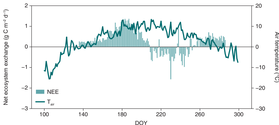
Figure 3.13 Diurnal net ecosystem exchange (NEE) and air temperature (T air ) measured in the fen in 2011.
