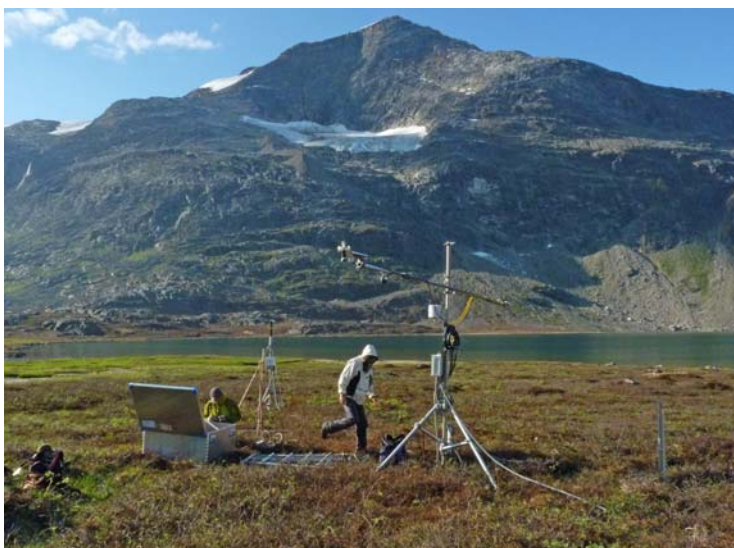
Figure 3.1 Two new energy balance stations were installed during 2011. One at a new heath site (upper) and one at the fen site (lower).
