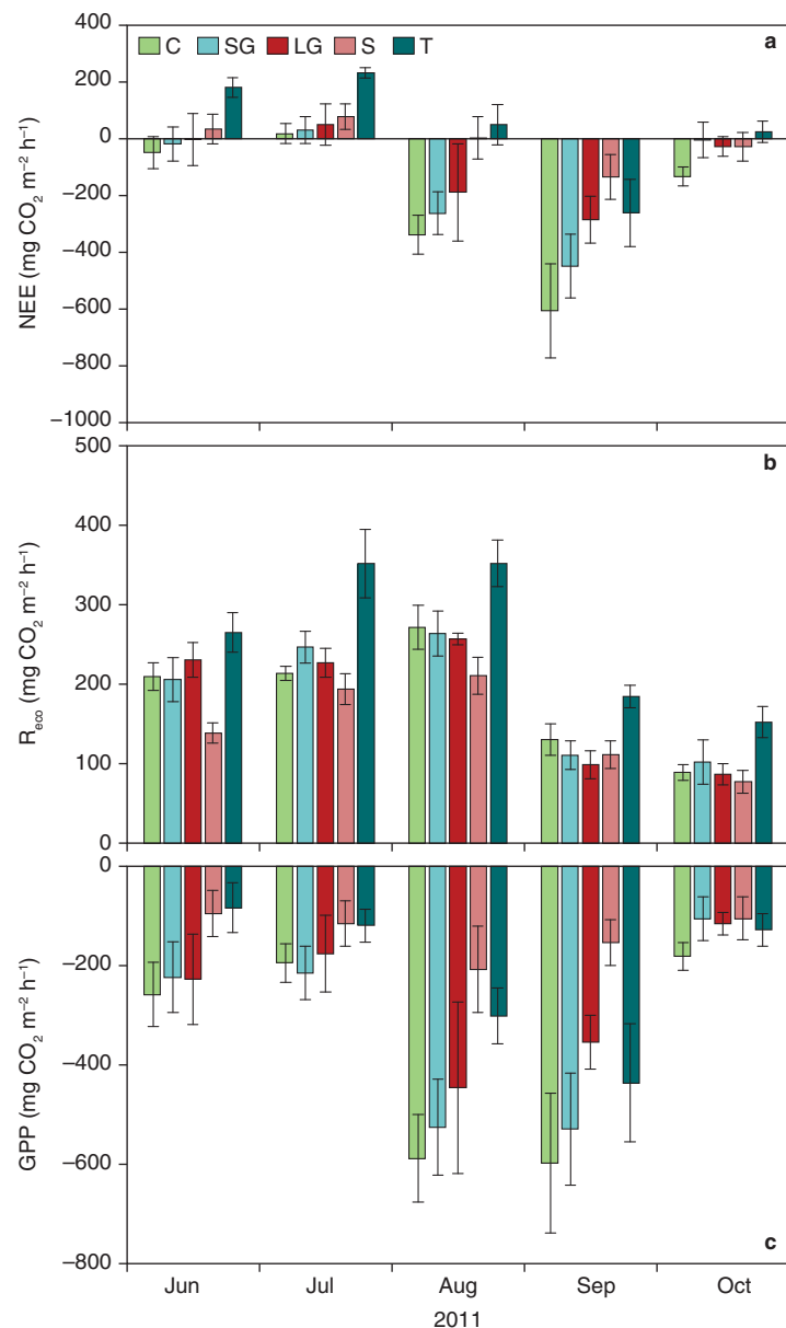
Figure 4.8 a) Monthly means of net ecosystem exchange (NEE), b) ecosystem respiration ( R_{eco} ) and c) gross primary production (GPP) in 2011 in the manipulation experiment. Error bars refer to standard error in spatial variability (six replicates). For explanation of treatment abbreviations, see the text.
