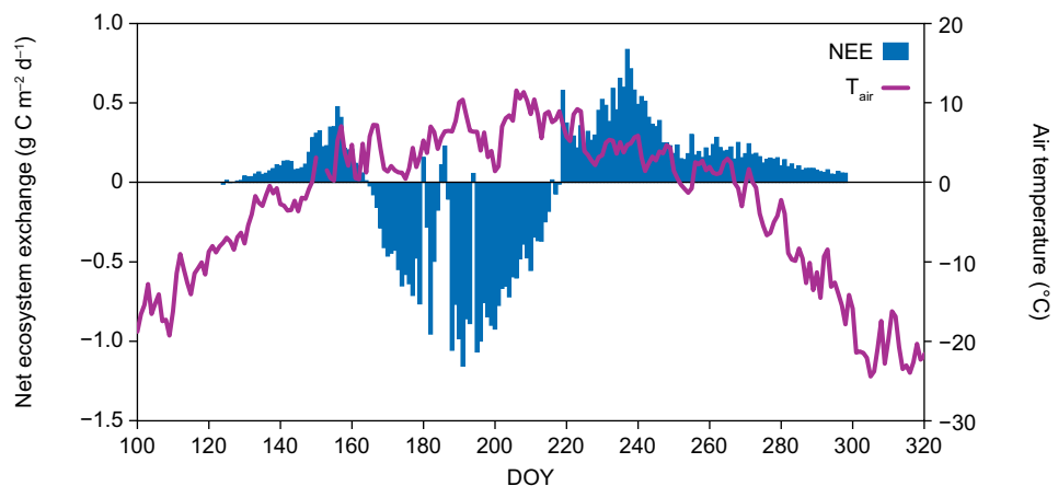
Figure 2.15 Daily net ecosystem exchange (NEE) and air temperature ( T_{\text{air}} ) measured at the heath site (MM1) in 2013.
