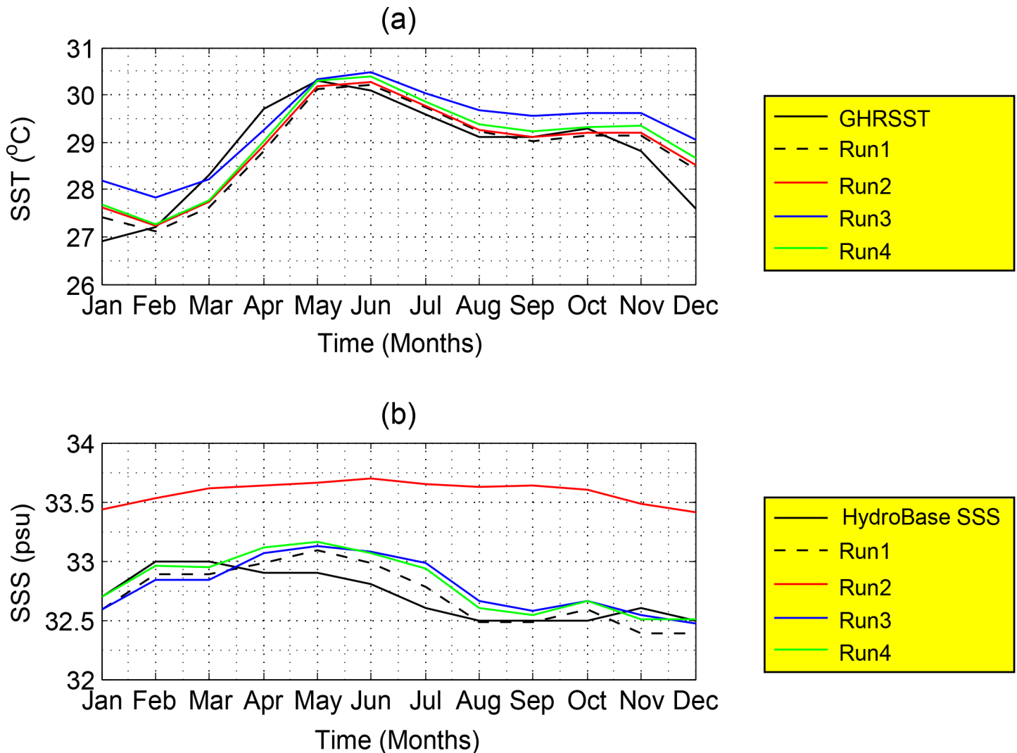
Fig 9. The mean monthly variations of SST (°C) and SSS (psu) represented for the GHRSSST and HydroBase SSS (the black lines), control run (Run1, black dashed-line), surface freshwater effect run (Run2, red line), wind stress effect run (Run3, blue line) and solar radiation effect run (Run4, green line).
