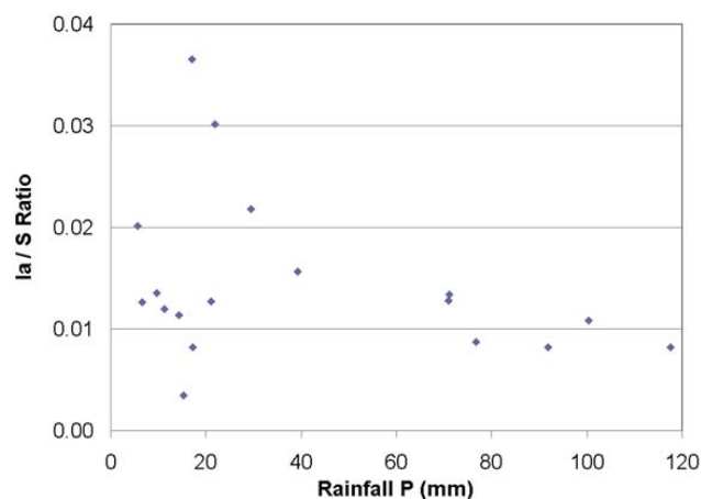
Fig. 2. Initial abstraction ratio Ia/S versus rainfall depth P , for each event.
