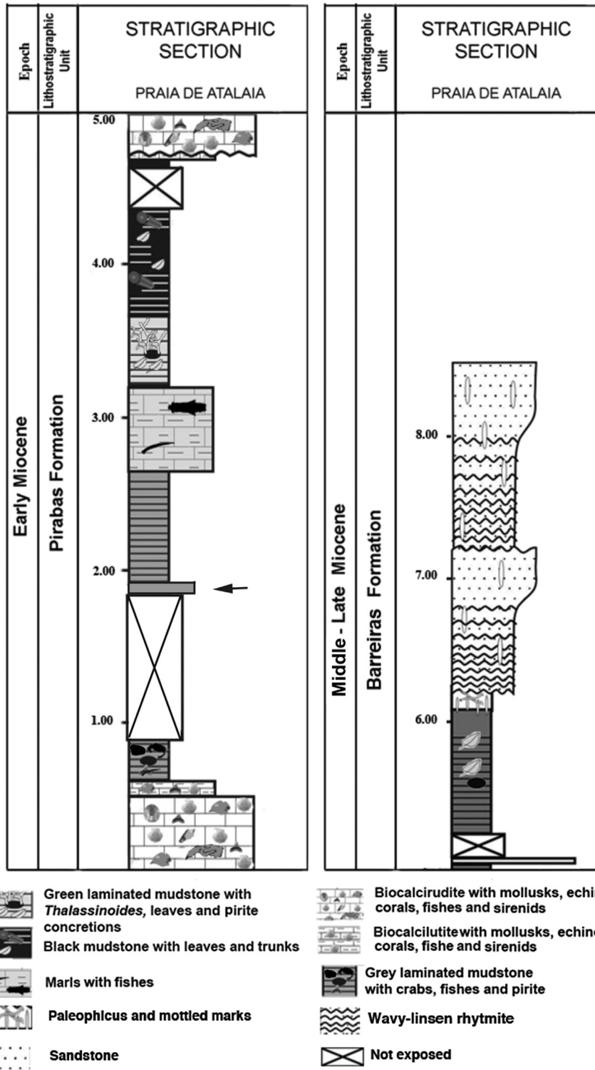
Fig. 2. Stratigraphic section of the Atalaia Beach outcrop. The arrow indicates the level with high otolith concentration. (base section modified from Aguilera et al., 2013a).
