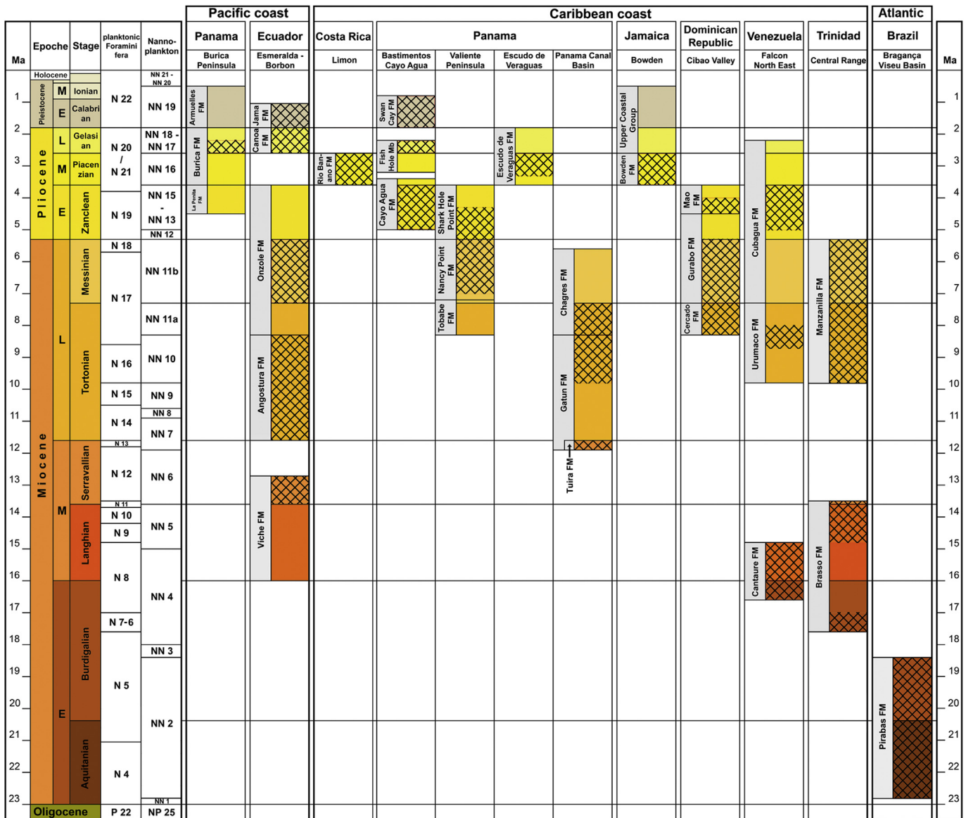
Fig. 3. Stratigraphic correlation chart depicting stratigraphic positions of otoliths studied (hatched) from Tropical America Neogene rocks (modified from Schwarzahns and Aguilera, 2013 with additional stratigraphy data from Brazil after Rossetti et al., 2013).
