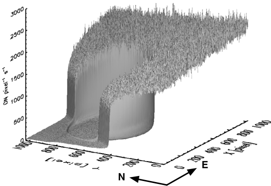
Fig. 3. Top panel: image ( 1024 \times 1024 pixels) of Venus (dark circular subaperture) transiting the Sun (brighter areas) on June 5, 2012 as seen by the Hinode SOT/SP spectropolarimeter (total intensity Stoke parameter I ) in the red filter centered at 6684.0 \pm 0.1 \text{ \AA} (red filter). The intensity range is 0. - 2.7 \times 10^3 \text{ DN pixel}^{-1} \text{ s}^{-1} (where DN is data number, Lites et al. 2013). The intensity plotted is the square root of the intensity to better display the “aureole”. Central panel: same figure as above with the contrast highly increased to fit the radius of the planet, yellow circle, with the procedure described in the text ( R_{\text{fit}} = 274.91 pixels). The center of the Sun is located in southeast direction. Bottom panel: three-dimensional view of the images above. The contribution of the aureole is visible in the region just outside the solar disk.
