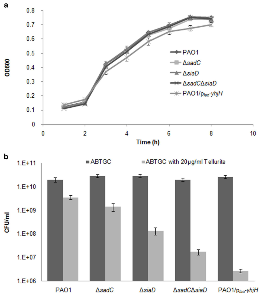
Figure 4. Growth curve (a) and TeO_3^{2-} tolerance assay (b). P. aeruginosa PAO1, \Delta sadC , \Delta siaD , \Delta sadC\Delta siaD , and PAO1/ p_{lac-yhjH} strains were cultivated in ABTGC medium at 37 °C with shaking for growth measurement. For TeO_3^{2-} tolerance assay, P. aeruginosa PAO1, \Delta sadC , \Delta siaD , \Delta sadC\Delta siaD , and PAO1/ p_{lac-yhjH} strains were cultivated in ABTGC medium with the presence of 20 \mu g/ml TeO_3^{2-} overnight followed by CFU determination. Means and standard deviations of three replicates are shown.
