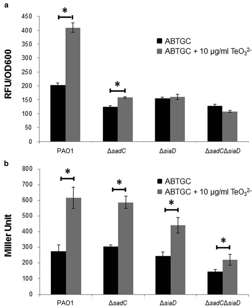
Figure 2. Expression of biosensor P_{cdrA-gfp} (a) and P_{pel-lacZ} (b) by P. aeruginosa strains in ABTGC medium with and without the presence of 10 µg/ml TeO_3^{2-} . The P_{cdrA-gfp} expression was shown as relative fluorescence units (RFU) per OD_{600} . The P_{pel-lacZ} expression was shown as Miller Unit. Means and standard deviations of three replicates are shown. Student's t -test was performed for testing differences between groups. * P < 0.05 .
