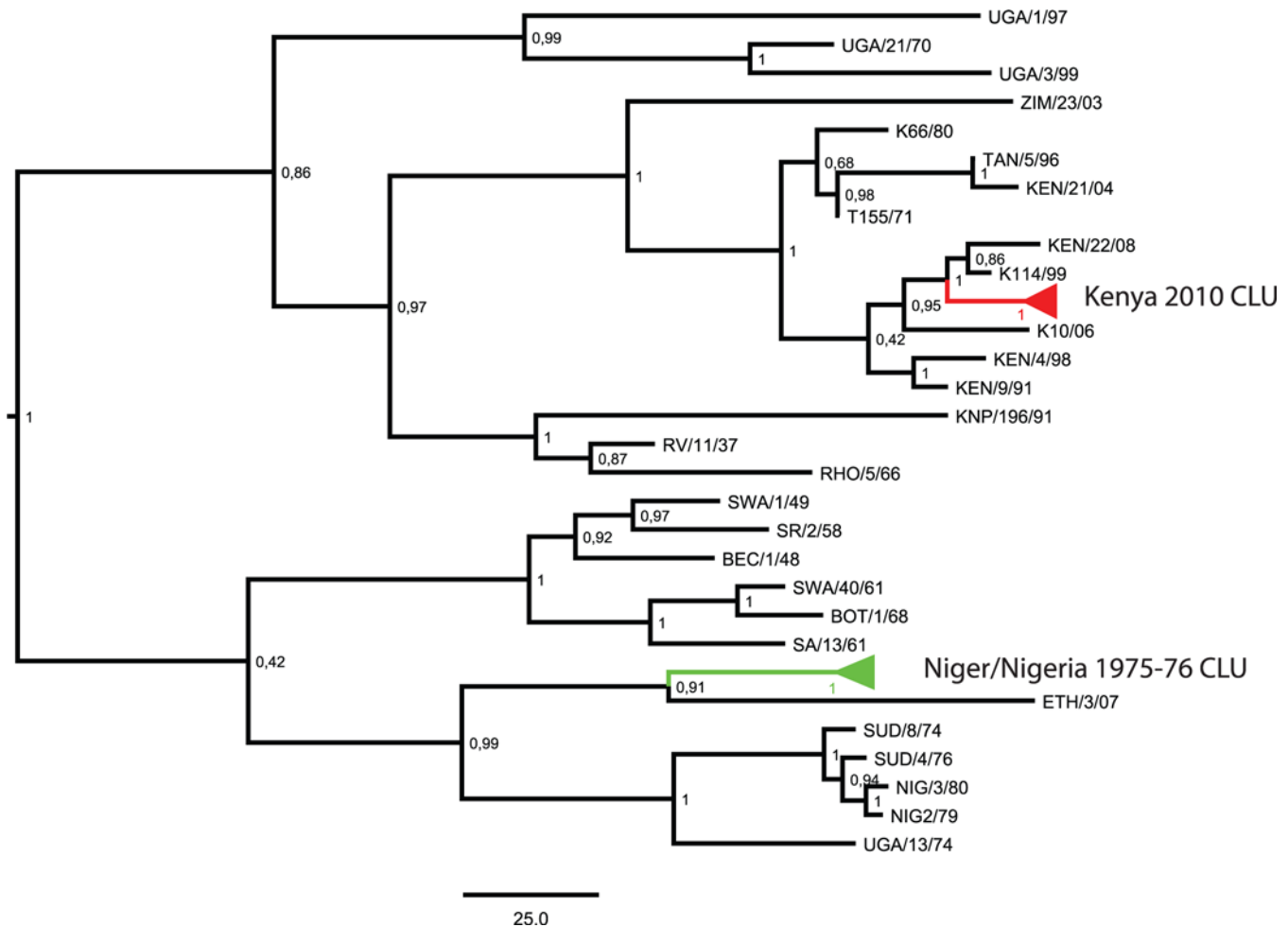
Fig 1. SAT 1 Phylogenetic Tree. Markov Chain Monte Carlo phylogenetic tree generated using the combined SAT 1 data set including both chronologically sampled (CHR) data sets and temporal sample clusters (CLU). Temporal sample clusters are collapsed and coloured. Posterior probabilities are given for each node and the scale bar indicates a branch length corresponding to 25 years.
