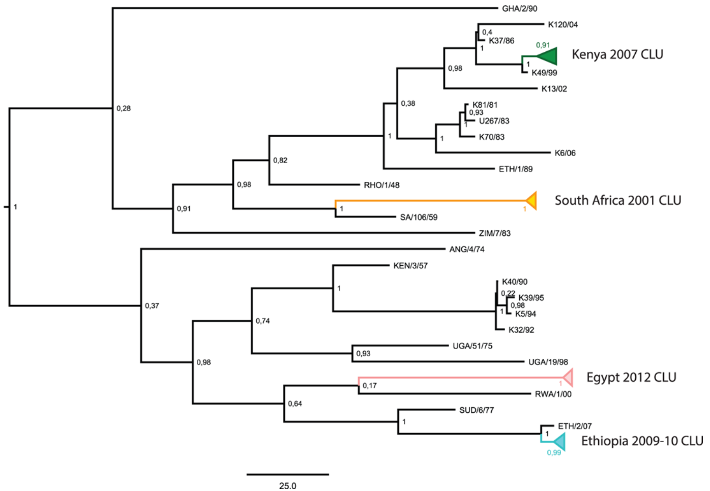
Fig 2. SAT 2 Phylogenetic Tree. Markov Chain Monte Carlo phylogenetic tree generated using the combined SAT 2 data set including both chronologically sampled (CHR) data sets and temporal sample clusters (CLU). Temporal sample clusters are collapsed and coloured. Posterior probabilities are given for each node and the scale bar indicates a branch length corresponding to 25 years.
