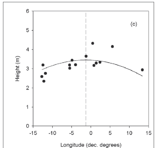
Fig. 2. Regressions of height growth with longitude at Dinderesso site, Burkina Faso.
