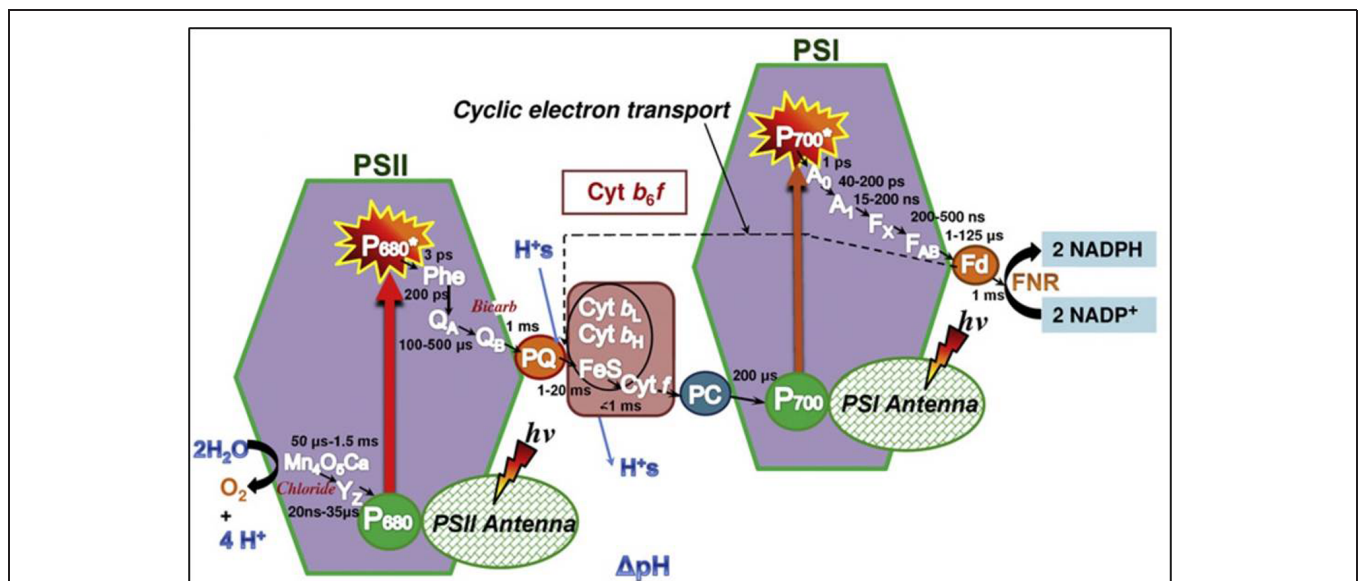
FIGURE 5 | The Z scheme, illustrating the photosynthetic electron transport chain from PSII via PQ to the cytochrome b 6 f complex. PC further conveys electrons to PSI, which facilitates the last part of the chain, resulting in reduction of NADP + to NADPH. Figure is from Stirbet and Govindjee (2011).
