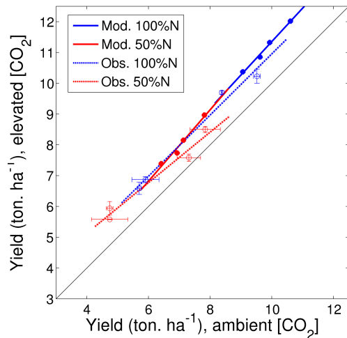
Figure 5. Effect of CO 2 fertilisation on observed and simulated grain yield, comparing wheat grain yields grown at elevated CO 2 (~ 548 ppm) with those grown at ambient CO 2 (~ 378 ppm). Simulated yields are depicted by solid lines and filled circles, observations are depicted by dashed lines and markers, shown for treatments with sufficient N fertiliser input (100 % N, blue), and treatments that received half of that amount (50 % N, red). Observations are from (Table 4 Weigel and Manderscheid, 2012).
