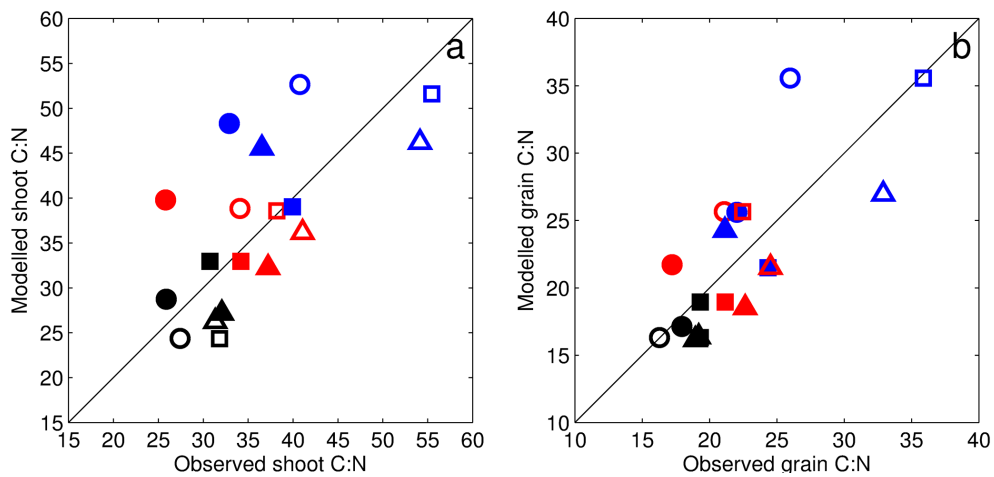
Figure 4. A comparison between modelled and observed C :N in harvested above-ground biomass (a) and grains (b), for the Eest, the Bouwing and PAGV, the Netherlands for the seasons 1982–1983 and 1983–1984. Symbols are the same as in Fig. 2 with blue symbols for low input of N fertiliser, red for a medium input of N and black for high N input.
