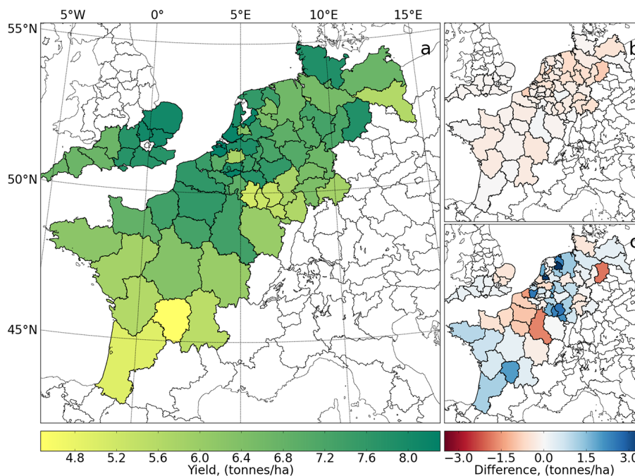
Figure 6. Reported regional yields from EUROSTAT (a), differences between simulated and reported yields for the F_{opt(T,A)} setup (b) and the F_{t,1} (c) simulations.
