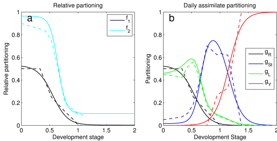
Figure 1. (a) The allocation to roots relative to vegetative organs ( f_1 ) and the allocation to leaves relative to leaves and stem ( f_2 ) for winter wheat. Dashed lines represent the allocation model from Penning de Vries et al. (1989) and solid lines are fitted Richards equations (Eqs. 3 and 4). (b) The resulting allocation scheme to roots ( g_R ), stem ( g_{St} ), leaves ( g_L ) and grains ( g_Y ) (solid lines) compared to data from Penning de Vries et al. (1989) (dashed lines) from equations in Eq. (6).
