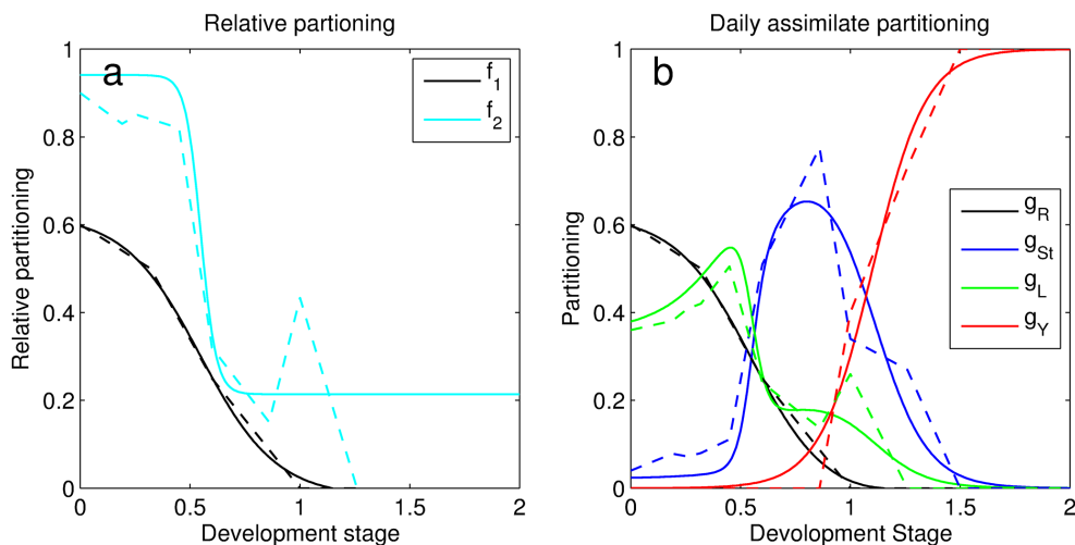
Figure A1. (a) The allocation to roots relative to vegetative organs ( f_1 ) and the allocation to leaves relative to leaves and stem ( f_2 ) for spring wheat. Dashed lines represent the allocation model from Penning de Vries et al. (1989) and solid lines are fitted Richards equations (Eqs. 3 and 4). (b) The resulting allocation scheme to roots ( g_R ), stem ( g_{St} ), leaves ( g_L ) and grains ( g_Y ) (solid lines) compared to data from Penning de Vries et al. (1989) (dashed lines) from equations in Eq. (6).
