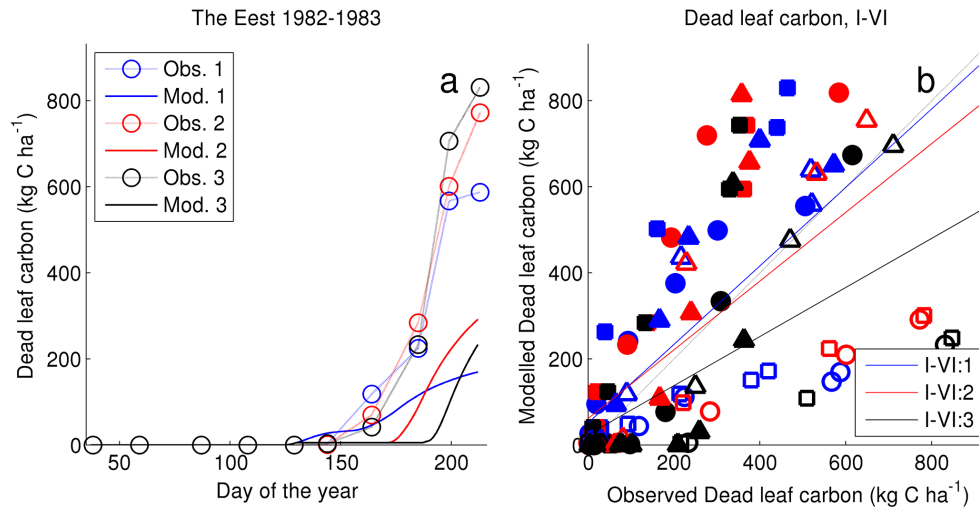
Figure A3. (a) Dead leaf comparison between modelled (thick lines) and observations for the Eest, the Netherlands 1982–1983. Blue lines are with 0 input of N fertiliser; red lines are with an input of 60 kg N ha -1 ; and black lines are with 160 kg N ha -1 . (b) A comparison between modelled and observed C mass of dead leaves for winter wheat for the Eest (○), the Bouwing (□) and PAGV (△), the Netherlands for the seasons 1982–1983 and 1983–1984. Blue symbols are with a low input of N fertiliser; red are with a medium input of N; and black are with a high input. Open symbols are for the season 1982–1983, and closed symbols are for the season 1983–1984.
