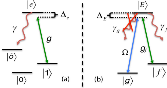
FIG. 1 (color online). (a) Level structure of the qubit atoms. Only state |1\rangle couples to the cavity and we assume that the excited level decays to some level |\tilde{0}\rangle , possibly identical to |f\rangle or |0\rangle . (b) Level structure of the auxiliary atom and the transitions driven by the weak laser ( \Omega ) and the cavity ( g_f ). We assume that |E\rangle \leftrightarrow |f\rangle is a closed transition, i.e., \gamma_g = 0 .
