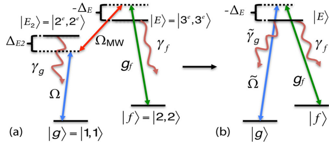
FIG. 3 (color online). (a) Level structure of the auxiliary atom and the transitions driven by a weak laser ( \Omega ), a microwave field ( \Omega_{\text{MW}} ), and the cavity ( g_f ). We assume that |E\rangle \leftrightarrow |f\rangle is a closed transition and, for simplicity, we also assume that |E_2\rangle \leftrightarrow |g\rangle is a closed transition but this is not a necessity. Here |r^{(e)}, r^{(e)}\rangle with r = 1, 2, 3 refers to how the atom may be realized in the ( 5^2P_{3/2} ) states |F^{(e)} = r, m^{(e)} = r\rangle 5^2S_{1/2} of Rb 87 . (b) Effective three-level atom realized by mapping the two-photon drive to give an effective decay rate \tilde{\gamma}_g and an effective drive \tilde{\Omega} .
