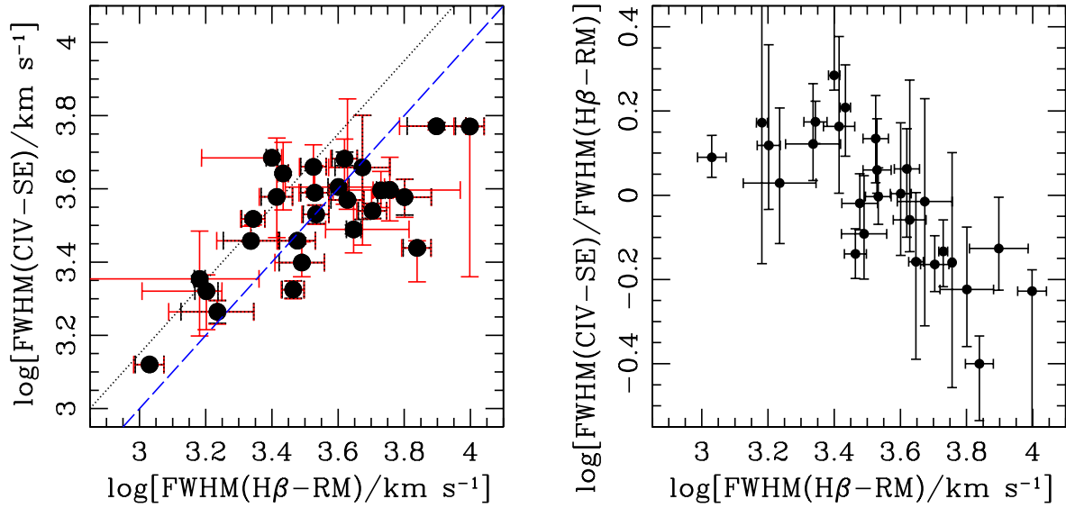
Fig. 12.— Relationship between the single-epoch CIV and H \beta line widths for the current sample. The H \beta data are the weighted average of the FWHM of the individual epoch spectra listed by Peterson et al. (2004). The CIV data points are likewise the weighted average of each FWHM entry in Table 2. ( Left ) The FWHM(CIV) and FWHM(H \beta ) are compared directly. The rms of the data points around the unity relation is 0.16 dex and relative to the black dotted relationship is 0.23 dex; the average “error bar” is 0.07 dex and 33% of the errors exceed 0.1 dex up to a maximum value of 0.41 dex. ( Right ) The ratio of line widths are compared to FWHM(H \beta ). See Figure 11 for symbols.
