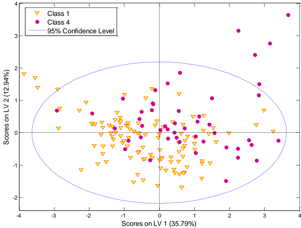
Figure 1. Scores Plot (LV1 vs. LV2) showing that lame cows tend to separate from non-lame towards the upper right quadrant. Class 1 – non-lame cow, Class 4 – extremely lame cow
