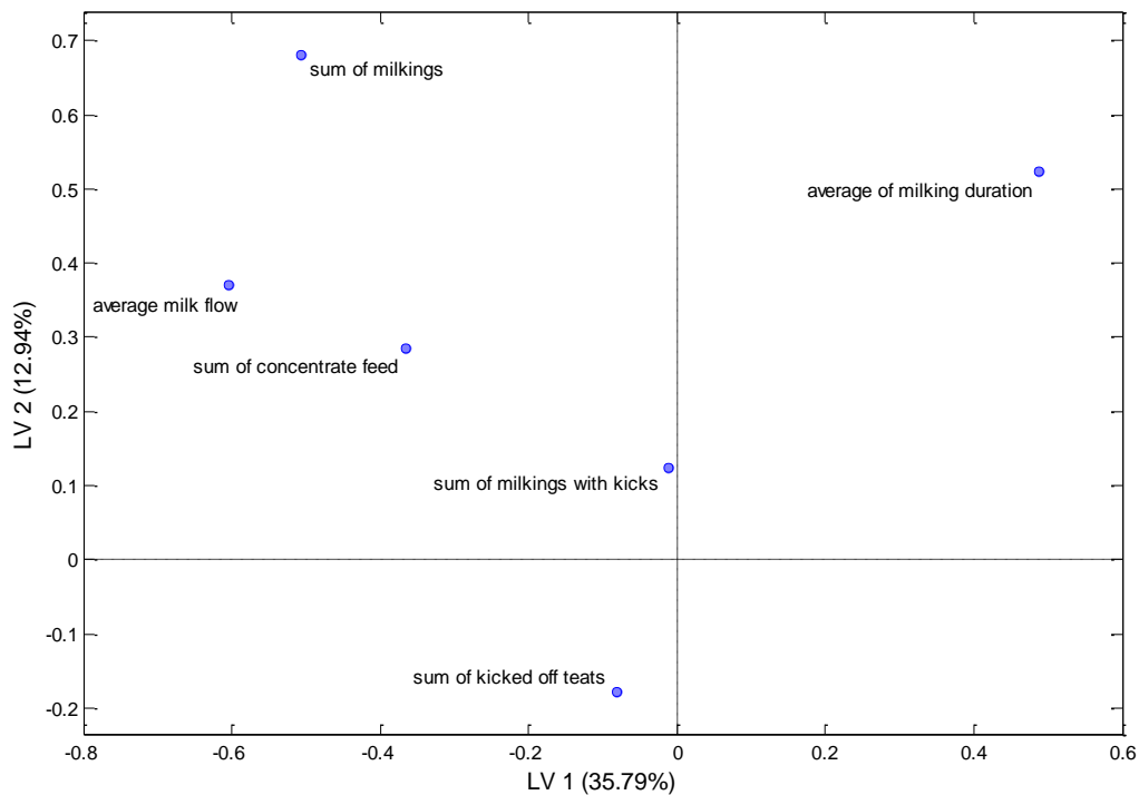
Figure 2. Loadings Plot (LV1 vs. LV2) showing that sum of milkings and average of milking duration are the variables that contribute the most to discriminate lame cows. Weekly variables: average of milking duration, sum of kicked off teats during milking, sum of milkings with kicks, average milk flow, sum of milkings and sum of concentrate feed in the robot.
