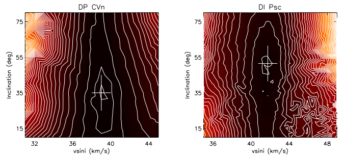
Fig. 6. Dependency of the normalized goodness-of-fit ( \chi^2 ) of our Doppler maps over the vsini - i parameter plane. Best values for DP CVn ( left ) are vsini of 39.0 \pm 1.0 km s ^{-1} with i \approx 35^\circ \pm 10^\circ and for DI Psc ( right ) are 42.0 \pm 1.0 km s ^{-1} with 50^\circ \pm 10^\circ , respectively.
