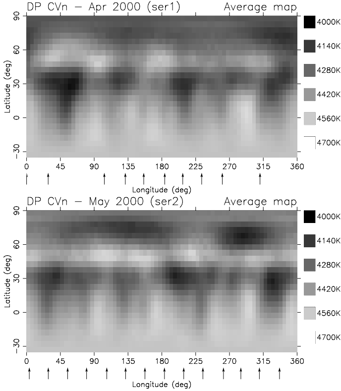
Fig. 8. Combined images of DP CVn for the two data subsets ser1 ( top ) and ser2 ( bottom ). The maps are presented in a pseudo-Mercator projection from latitude -35^\circ to +90^\circ . The phases of the observations are marked by arrows below the maps. Note, that even if the individual reconstructions show differences (cf. Fig. 7), the average maps still retain most of the traits.
