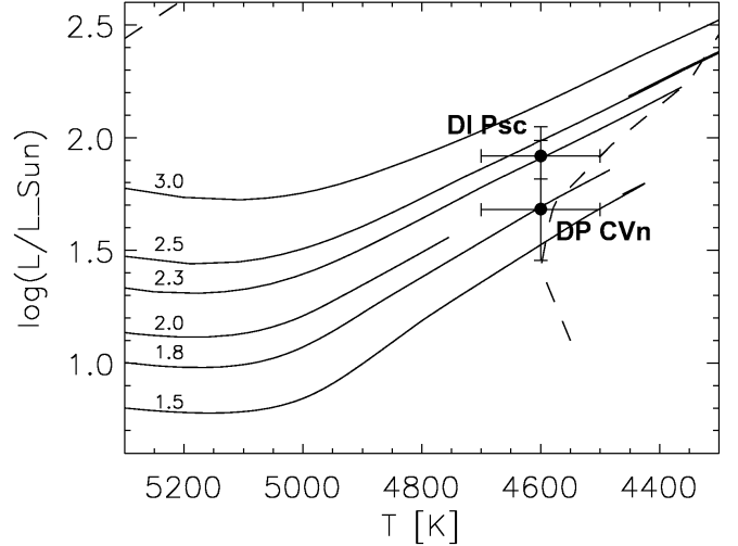
Fig. 1. Observed positions of DP CVn and DIPsc in the Hertzsprung-Russell diagram. The post-main-sequence tracks for 1.5, 1.8, 2.0, 2.3, 2.5 and 3.0 solar masses are shown (cf. Granzer et al. 2000). These tracks suggest masses of 1.8 M_\odot and 2.3 M_\odot for DP CVn and DIPsc, respectively. Both stars appear on the RGB at the end of the first Li dredge-up phase, which is marked by the dashed lines taken from Charbonnel & Balachandran (2000).
