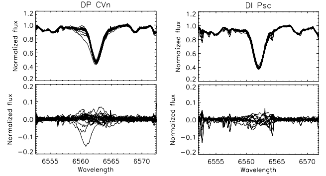
Fig. 5. H\alpha line profiles of DP CVn ( left ) and of DI Psc ( right ). In the top panels the observations are plotted together, while in the bottom panels the corresponding averages are subtracted to emphasize the night-time variations. Note the telluric water lines, especially at around 6552.5 Å, 6557 Å, and 6564 Å, as well as the sporadic cosmic peaks.
