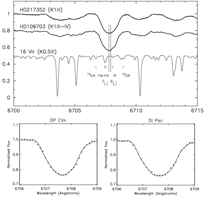
Fig. 4. Top panel: Li I 6708 Å spectra of DI Psc ( top ) and DP CVn (shifted by -0.2 ). Also shown is a spectrum of the inactive K0.5III giant 16 Vir (shifted to bottom ) for comparison purpose. The measured equivalent width of the lithium line of DI Psc and DP CVn is 328 \pm 5 mÅ and 316 \pm 7 mÅ, respectively. Bottom panels: Li I 6708 Å line fitted by synthetic spectra for DP CVn ( left ) and DI Psc ( right ), resulting in logarithmic abundances of \log n(\text{Li}) = 2.28 , and of 2.20, respectively.
