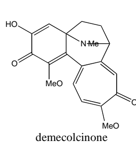
Fig. (10). Structural diversity of miscellaneous phenethylisoquinoline alkaloids in Colchicaceae.
