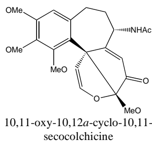
Fig. (10). Structural diversity of miscellaneous phenethylisoquinoline alkaloids in Colchicaceae.
