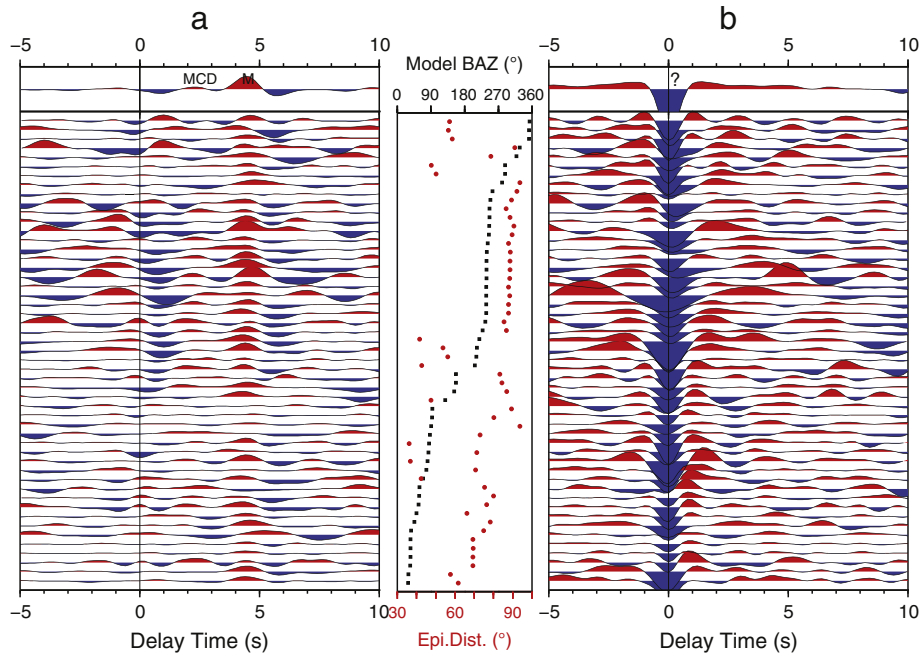
Fig. 6. P sv -RFs of station SA75 calculated a) using real incidence angles and b) assuming theoretical angles. The figure illustrates the improvement achieved from using real instead of the theoretical angles where artifacts are generated by complex crustal velocity structure that significantly deviate from the assumed reference model.
