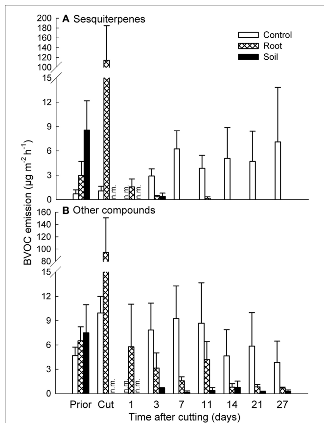
FIGURE 2 | Effect of experimental manipulations on biogenic volatile organic compound (BVOC) emissions from mixed heath mesocosms.
