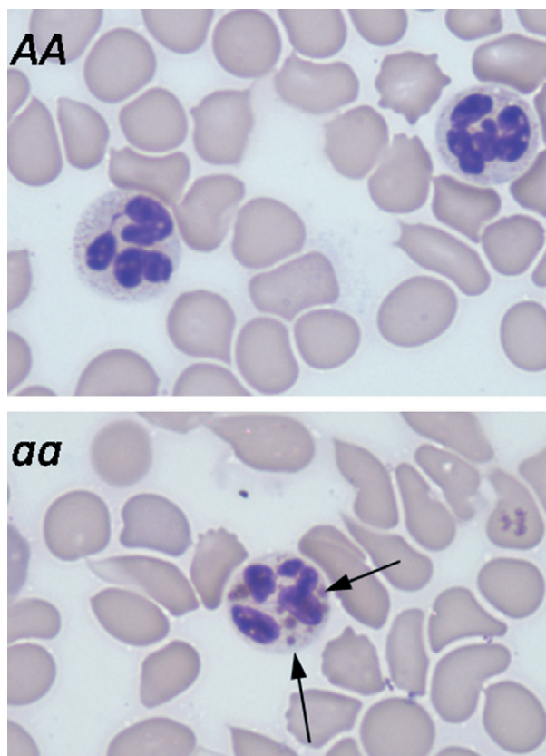
Figure 2 AA . Normal neutrophils from a peripheral blood smear of wild-type mink; aa . Neutrophils of Aleutian mink displaying giant granules.
