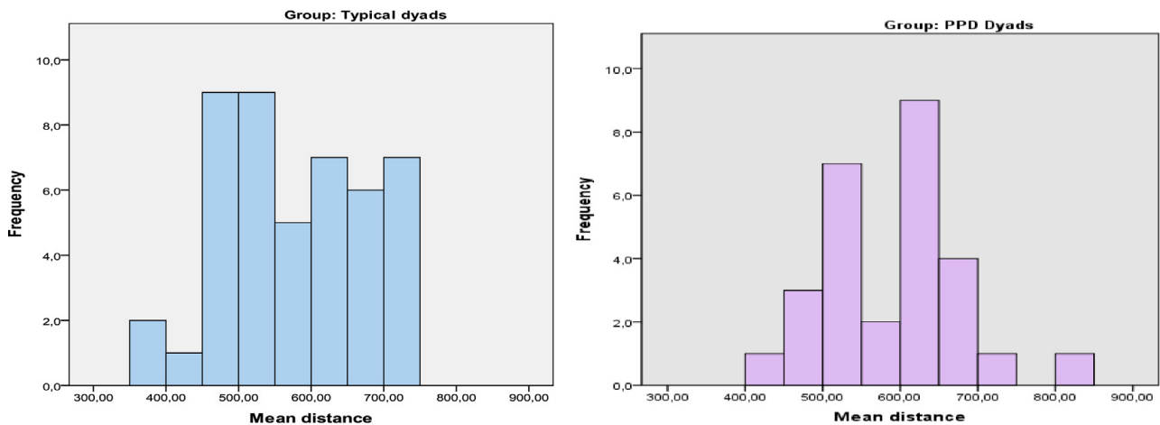
Fig. 2. Tables of means of spatial proximity for the two groups.
