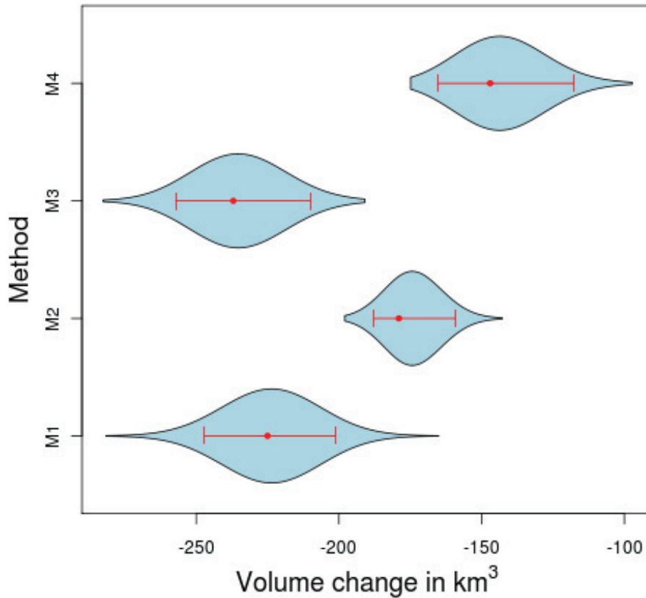
Fig. 2. Violin plot of the 4 method results. The blue area indicates the distribution of 1000 bootstrap samples. The red dots are the point estimates of volume change, and the red bars indicate the 95% confidence interval.
