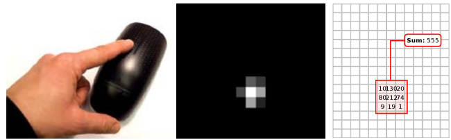
Figure 2: Interaction representation.
