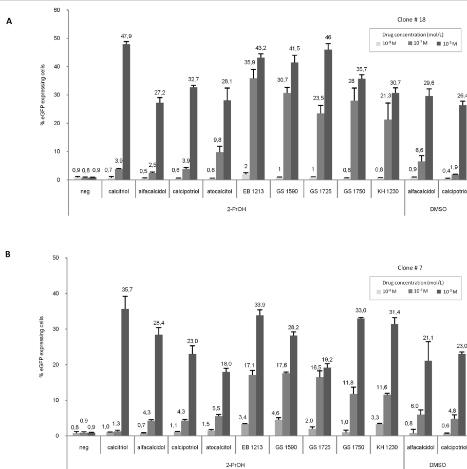
Figure 4 Sensor-based screening of 10 vitamin D3 analogues revealed compounds more potent than therapeutically approved drugs. (A) Efficacious sensor induction in clone #18. Cells derived from Clone #18 were exposed to vitamin D3 analogues at concentrations 10 -9 M, 10 -7 M and 10 -5 M. As indicated below the chart, the vitamin D3 analogues had been dissolved in either isopropanol (2-PrOH) or DMSO. After 48 hours the percentage of d2eGFP positive cells was measured by flow cytometry. Untreated (neg) cells served as control. A clear dose-dependent outcome is visible for all drugs. The experiment was conducted in triplicate, and data are indicated as mean values ± standard deviations. (B) Sensor induction in clone #7. Cells from clone #7 were treated as described for clone #18. The overall tendency is highly similar for clone #7 and #18.
