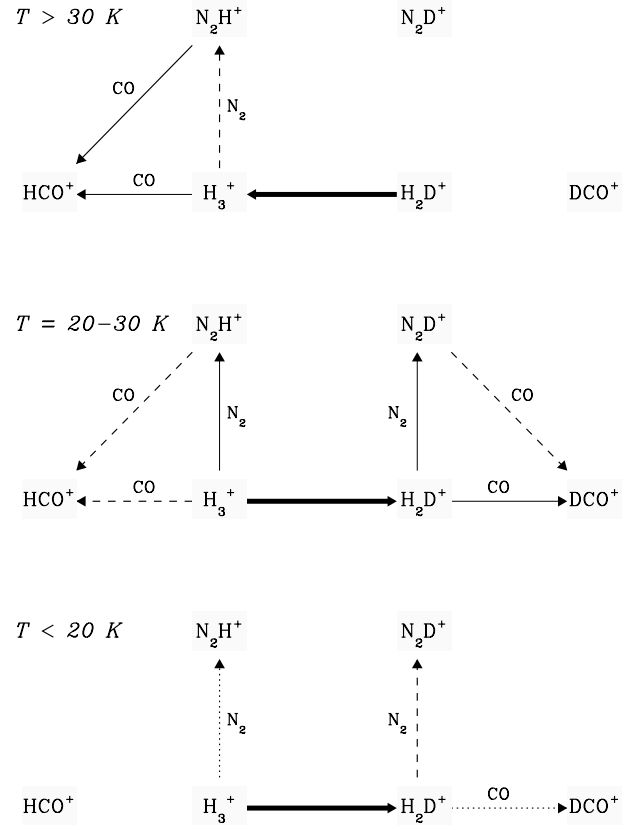
Fig. 18. Schematic chemical network for HCO^+ , DCO^+ , N_2D^+ and N_2H^+ in different regions of protostellar envelopes: at high temperatures ( T > 30\text{ K} ) CO is in the gas-phase and H_3^+ is dominating over H_2D^+ (the reaction in Eq. (1) proceeds to the left ) enhancing HCO^+ and destroying N_2H^+ . At intermediate temperatures ( T = 20\text{--}30\text{ K} ) CO depletion and H_2D^+ production starts to kick-in (the reaction in Eq. (1) proceeds to the right ), enhancing N_2H^+ (less destruction through CO) and the deuterated species ( DCO^+ in particular, through reactions between H_3^+ and CO). At low temperatures CO depletion is very significant and N_2D^+ is enhanced relative to the other species.
