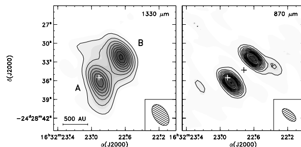
Fig. 1. Continuum images of IRAS 16293-2422 at 1.3 mm (left) and 0.87 mm (right). In the left panel the contours are given in steps of 0.1 \text{ Jy beam}^{-1} to 1.0 \text{ Jy beam}^{-1} and from there in steps of 0.2 \text{ Jy beam}^{-1} and in the right in steps of 0.2 \text{ Jy beam}^{-1} to 2.0 \text{ Jy beam}^{-1} and from there in steps of 0.4 \text{ Jy beam}^{-1} (in the continuum data the noise level is determined by the interferometer dynamic range). The white plus-signs indicate the pointing centers of the observations, except those from 2007 March 22 for which the pointing center is indicated by the black plus-sign in the right panel.
