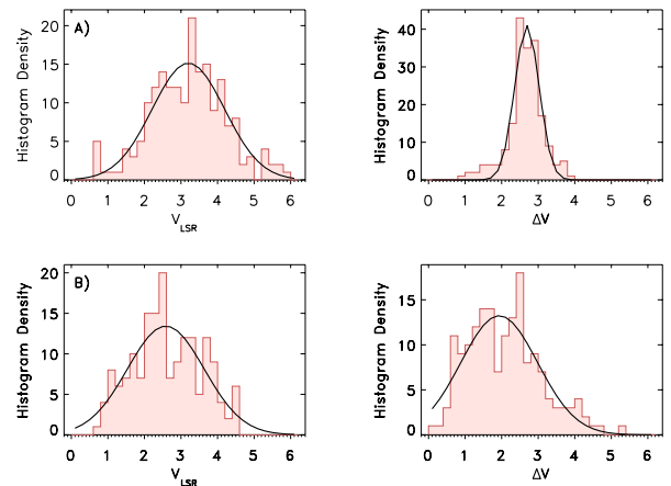
Fig. 11. Distribution of centroid velocities and widths (dispersions) in the left and right panels, respectively for emission lines detected toward the A source ( upper panels ) and B source ( lower panels ). Gaussian fits to the distributions are over-plotted ( V_{\text{LSR}} of 3.2 and 2.7 km s -1 and \Delta V of 2.6 and 1.9 for A and B respectively). The V_{\text{LSR}} and \Delta V distributions for the two sources are significantly different according to a standard T test for distributions with unequal variances.
