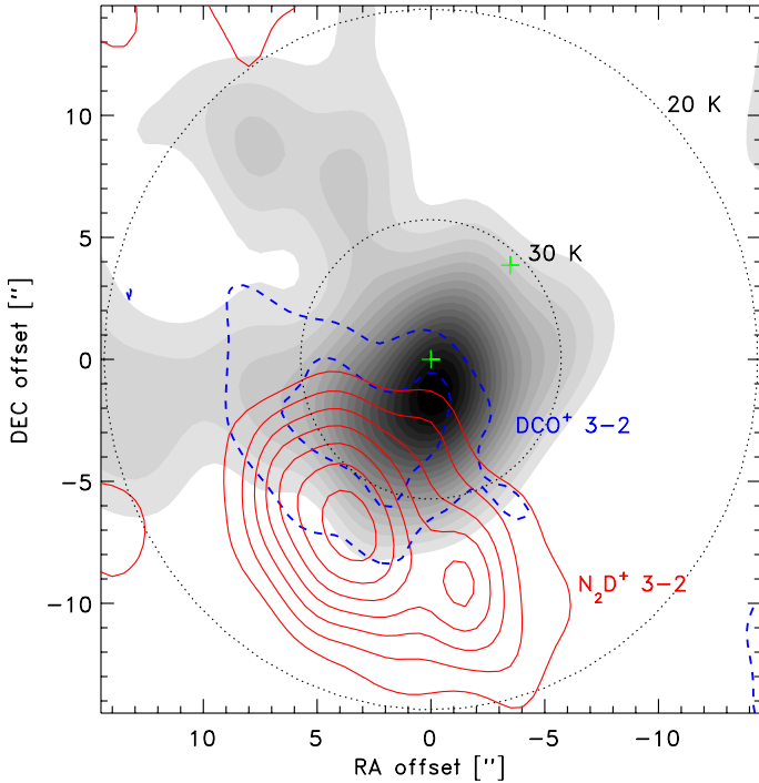
Fig. 17. Comparison between the C^{18}O 2–1 (grey-scale), DCO^+ 3–2 (dashed blue contours) and N_2D^+ 3–2 toward the core. The lines are integrated from velocities of 3\text{--}7\text{ km s}^{-1} ( C^{18}O and N_2D^+ ) and 4\text{--}6\text{ km s}^{-1} ( DCO^+ ). The dotted circles indicate the projected radii, where the dust temperature from radiative transfer calculations (Schöier et al. 2002; Jørgensen et al. 2005a) has dropped to 30 K and 20 K, respectively – assuming that the IRAS 16293A component is the sole source of luminosity and that the envelope is centered on this source.
