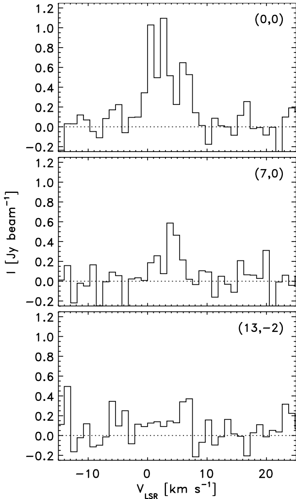
Fig. 22. Representative spectra of HDO in the central beams from maps with a 3'' taper applied (see also Fig. 21) toward the continuum peak of IRAS 16293A, the secondary peak and a position further offset toward the east where the emission is extended the offsets relative to the position of IRAS 16293A in arcseconds given in the upper right corner of each panel.
