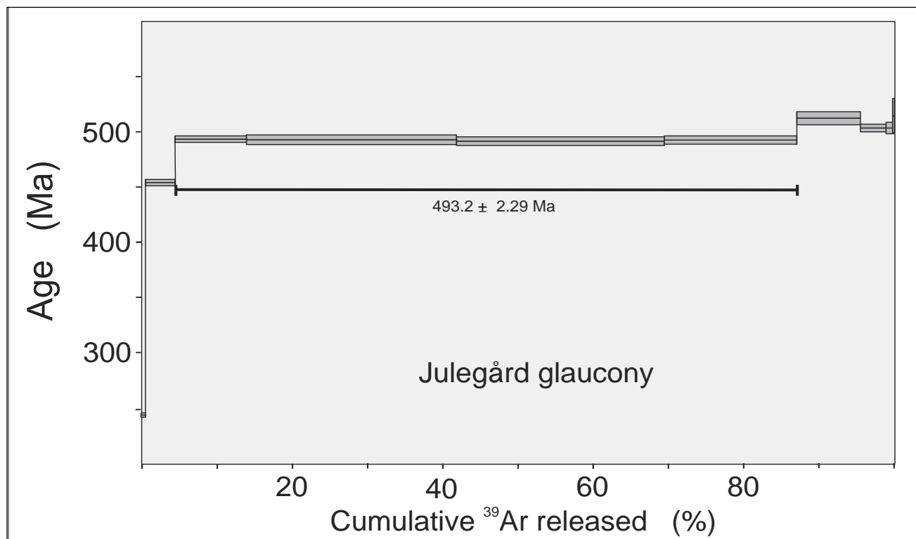
Fig. 9. Age spectrum for stepwise ^{40}\text{Ar} - ^{39}\text{Ar} analysis of glaucony from the marine deposits at Julegård, south coast of Bornholm.
