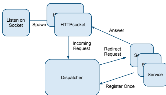
Figure 2. Webserver PyCSP design
