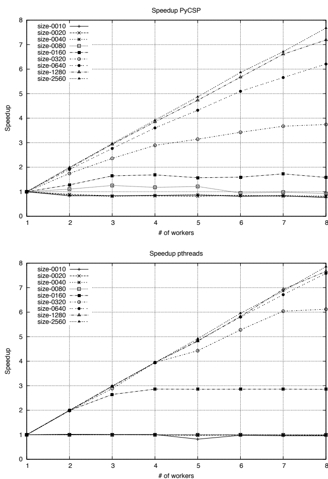
Figure 4. Speedup of PyCSP and Pthreads Mandelbrot computations.
