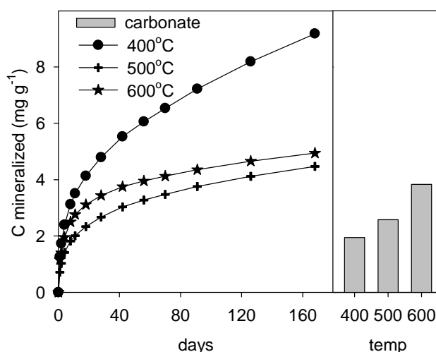
Figure 1. Mineralization of C and C in carbonates of biochars produced at 400°C, 500°C and 600°C.
