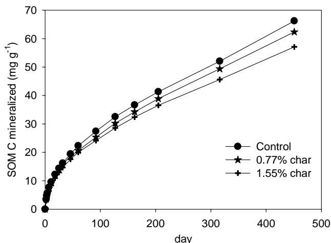
Figure 2. Mineralization of SOM C from a control soil and soils amended with different amounts of biochar
