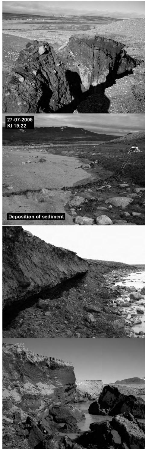
Fig. 2.19. Photos showing erosion along Zackenbergelven and at the delta cliff as a response of the flood 25 July.
