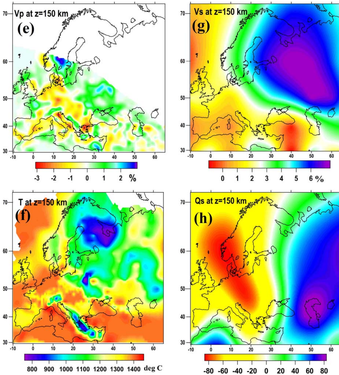
Fig. 2. Cross-section of the European lithosphere at depths of 150 km and 250 km (continued).
