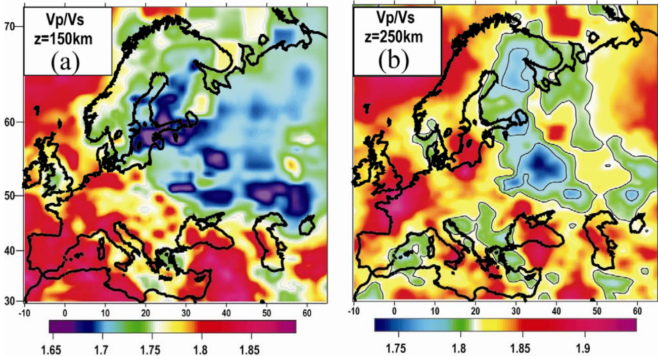
Fig. 10. Compositional anomalies in the lithosphere of Europe, i.e. anomalies of Vp/Vs ratio at depths of 150 km and 250 km calculated from smoothed and filtered P-wave tomography model by Bijwaard & Spakman (2000) recalculated to absolute velocity by scaling by ak135 model values and S-wave tomography model by Shapiro & Ritzwoller (2002a, b). Vp/Vs ratio is thought to be more sensitive to compositional than temperature variations (e.g. Lee 2003). Note low lateral resolution for north-eastern parts of the maps due to low resolution of the P-wave tomography model (compare with Fig. 2a, c).
