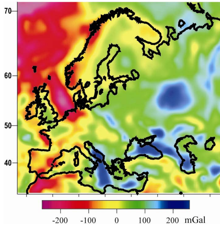
Fig. 5. Mantle residual gravity anomalies, which are a part of a 3D global model (Kaban et al. 1999 2003; Kaban & Schwintzer 2001), supplemented by higher resolution regional data (Kaban 2001). The anomalies reflect density variations produced by compositional or temperature variations, presumably in the upper 40–60 km of the subcrustal lithosphere.
