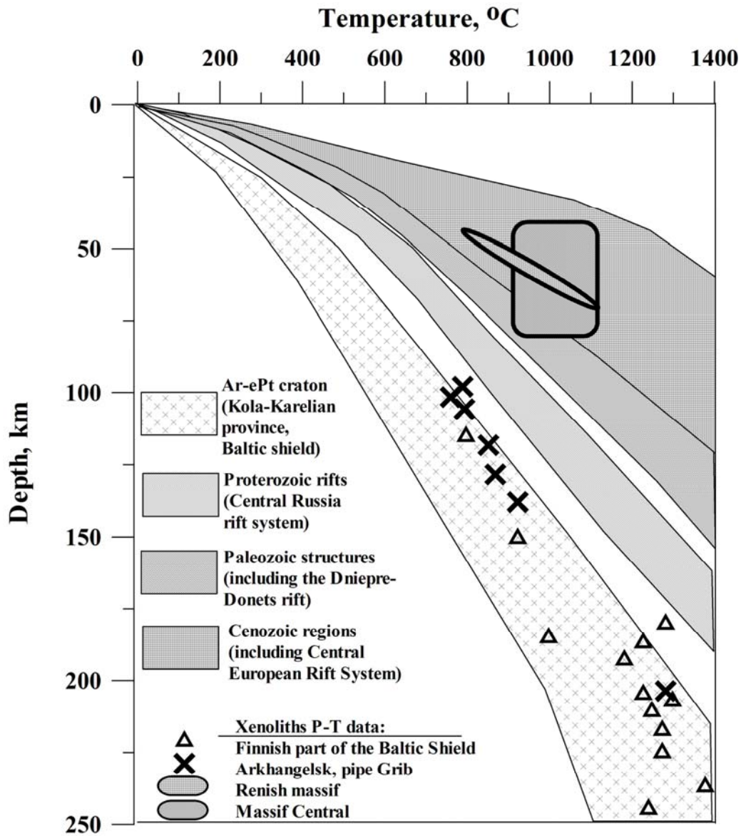
Fig. 6. Typical geotherms in different tectonic structures of Europe. For stable parts of the EEC the geotherms are constrained by surface heat flow data assuming steady-state conductive regime (Artemieva 2003).
