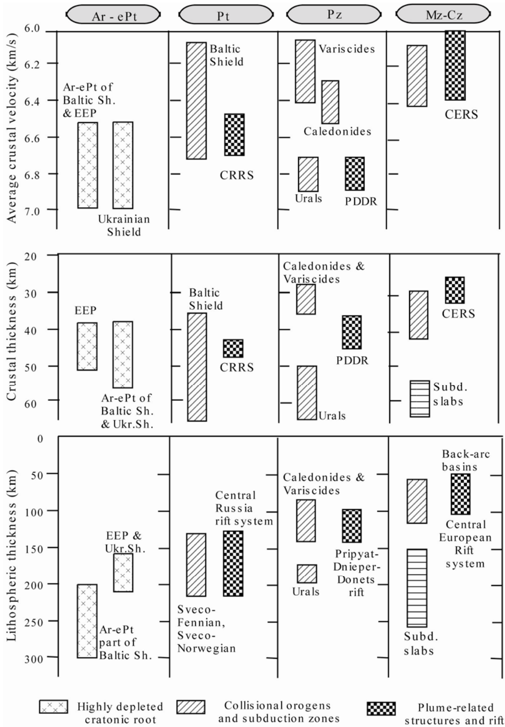
Fig. 7. Ranges of (a) average V_p seismic velocities in the crust, (b) crustal thickness, and (c) lithospheric thickness in different tectonic structures of Europe (based on Table 1).
