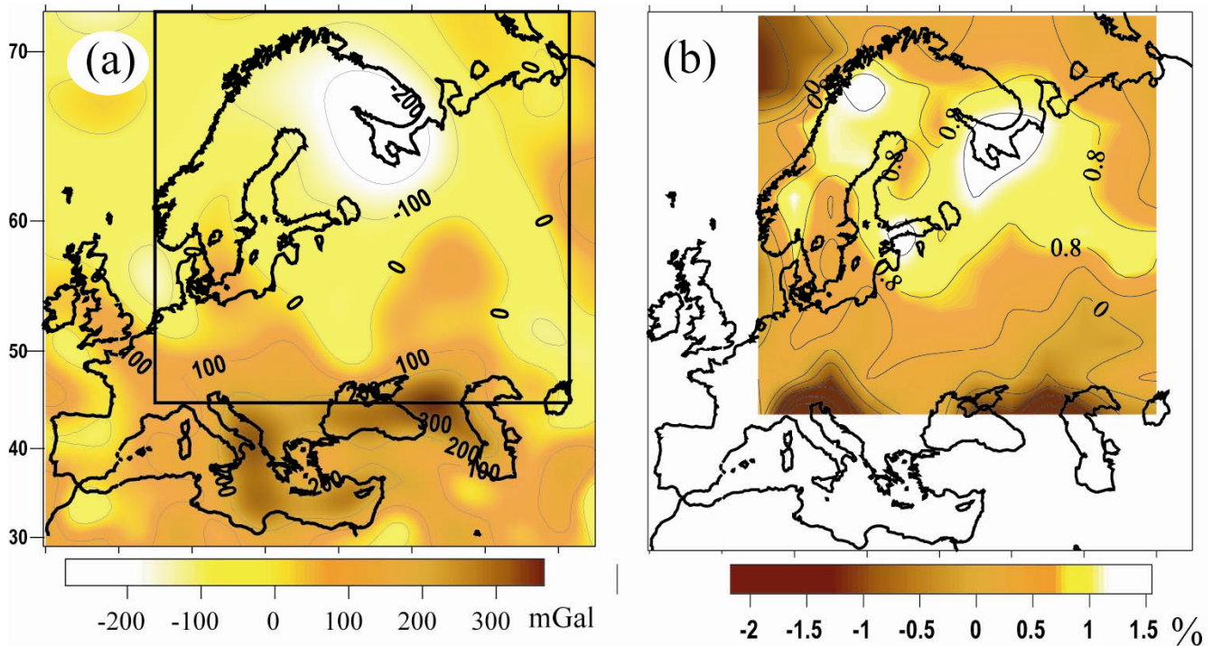
Fig. 11. Density anomalies in the upper mantle of Eurasia of a non-thermal origin.
