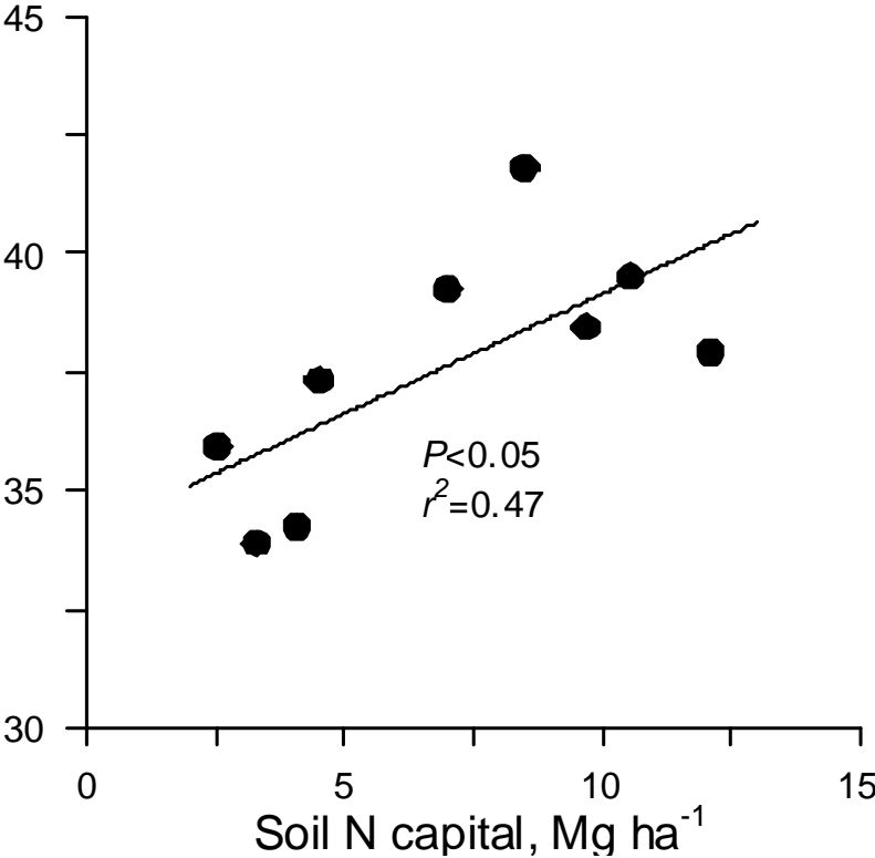
Fig. 5. Forest floor C/N ratios along the gradient in soil N capital.
