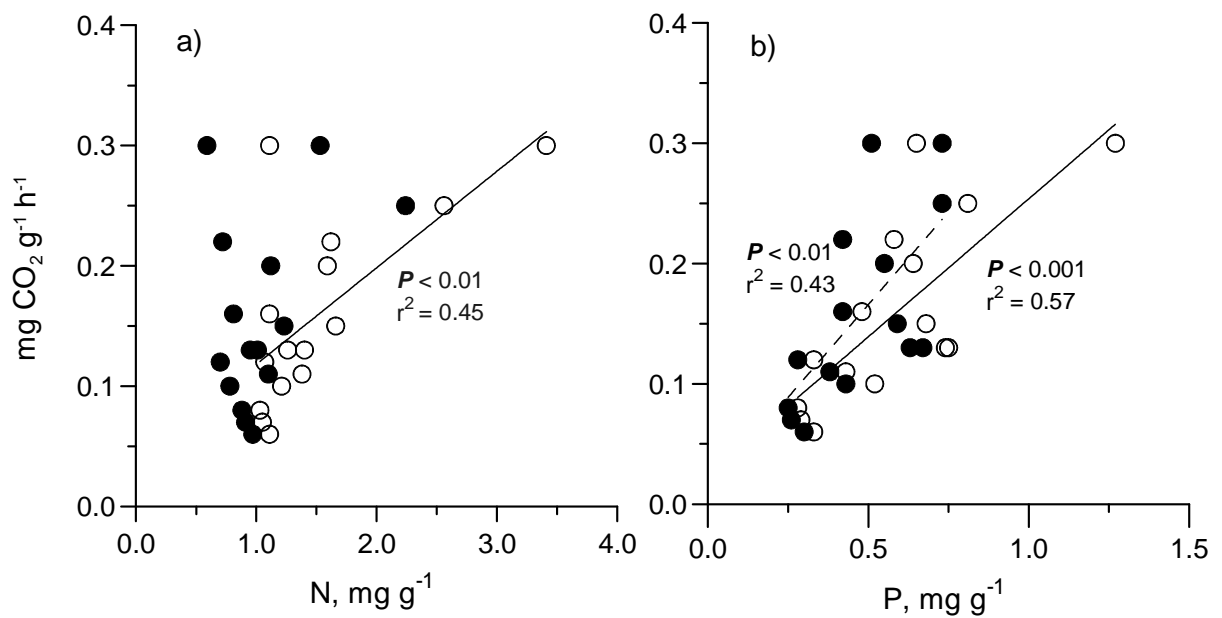
Fig. 5. a) Correlations between basal respiration rate and N availability in the forest floor. b) Correlations between basal respiration rate and P availability in the forest floor. ○ and — , uncorrected availability; ● and - - - - - , SIR corrected availability.
