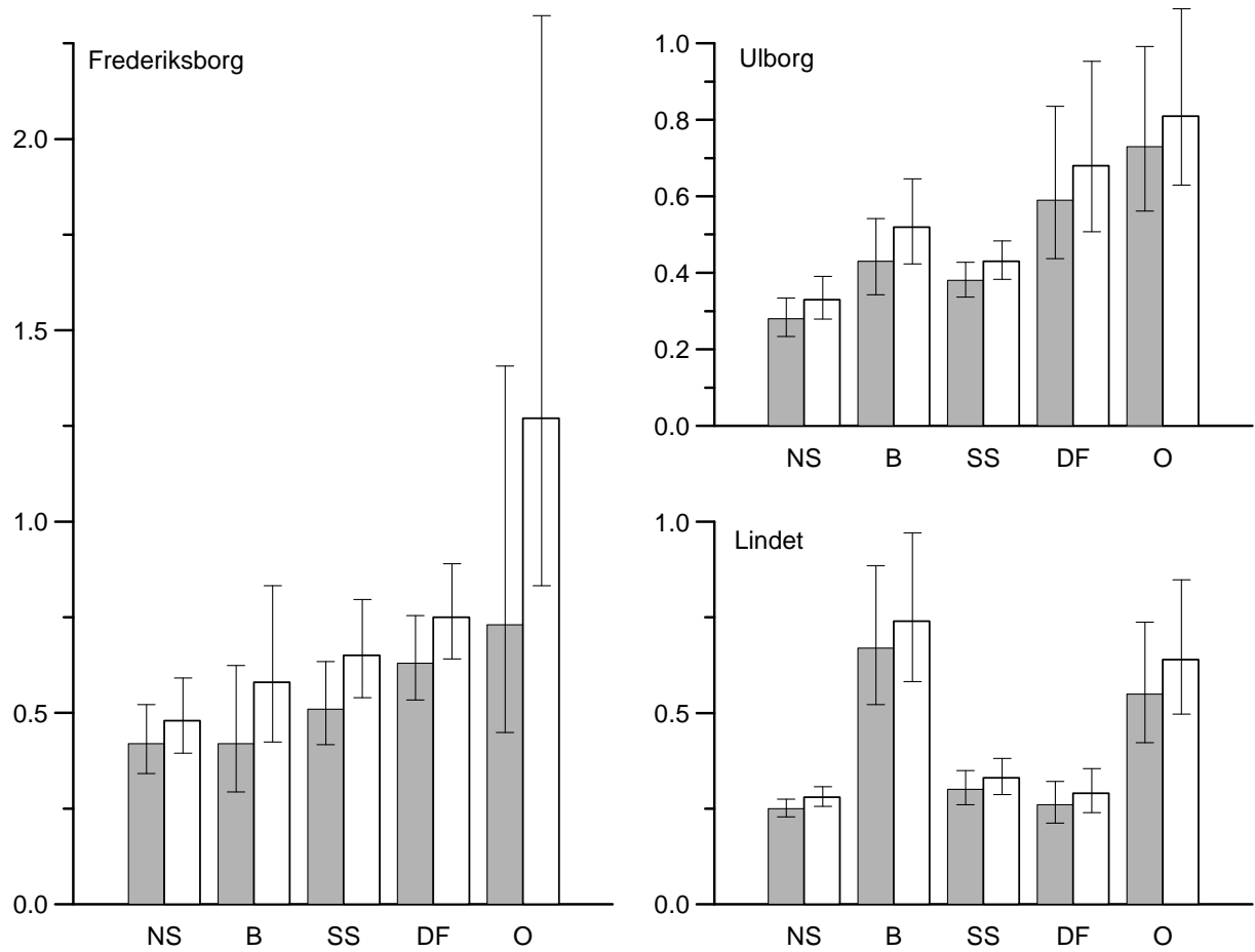
Fig. 4. Potential microbial P availability (mg g -1 ). Shaded bars are SIR corrected P availability. Error bars are 95% confidence intervals. Tree species legend as in Fig. 2.
