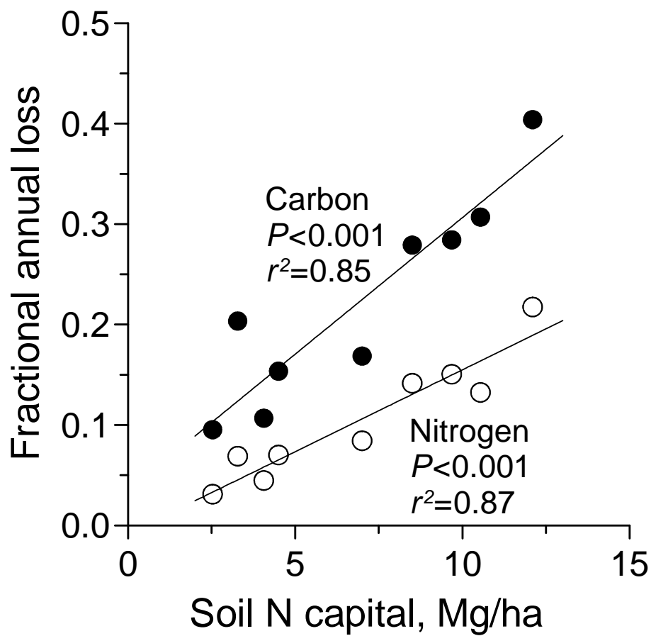
Fig. 3. Turnover rate constants ( k ) for carbon and nitrogen along the gradient in soil N capital. The slopes of the regression lines are significantly different ( P < 0.05 ).
