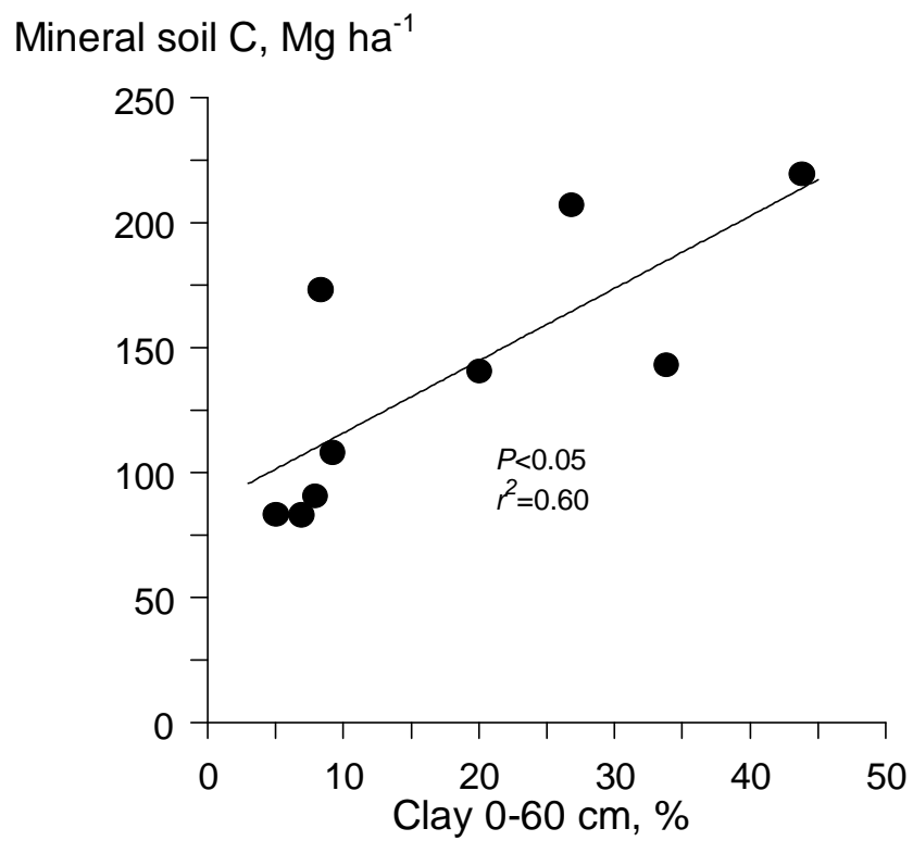
Fig. 7. The relationship between mineral soil carbon content and horizon-weighted percentage clay in 0-60 cm depth.
