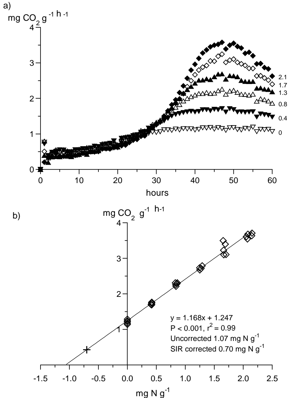
Fig. 1. Determination of potential microbial N availability in forest floor material from Norway spruce at Ulborg. a) average respiration rates (n = 5) resulting from different additions of N (mg (g dw) -1 ) together with glucose and P in excess. Substrate induced respiration rate (SIR) is the stable respiration rate attained immediately after start of the experiment. b) regression based on the obtained limited respiration rates. SIR is indicated by +.
