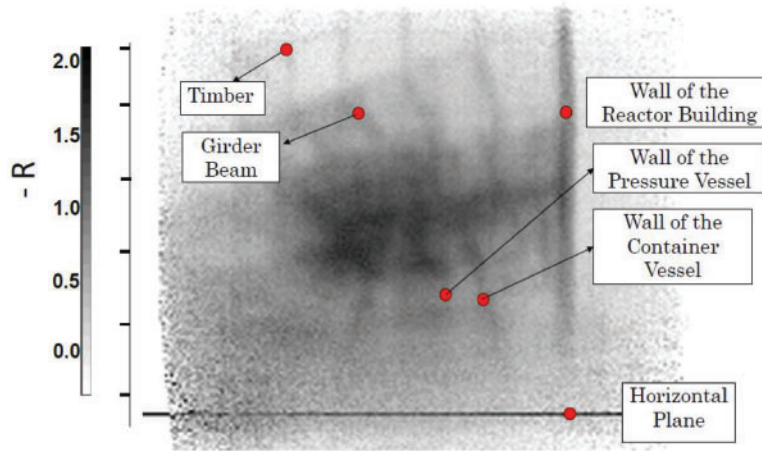
Fig. 6. Image of the reactor complex obtained from 15 million muons observed at MT1-1. The darkness, corresponding to the magnitude of the attenuation of the muon flux, is defined in the text.
