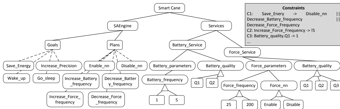
Figure 4. Feature model of the DSPL of the Smart Cane Platform.
