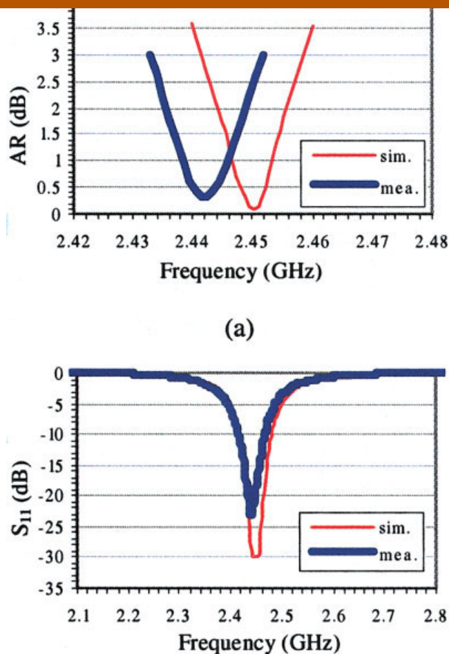
Figure 9 Results for (a) axial ratio and (b) return loss. [Color figure can be viewed in the online issue, which is available at www.interscience.wiley.com .]
