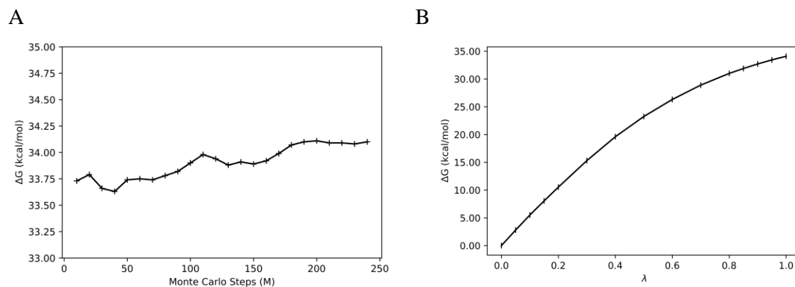
41 42 Figure 5. Electrostatic decoupling for the bound state after 80M configurations of equilibration. 43 (A) Evolution of the free energy change with simulation length. (B) Total free energy change as a 44 function of \lambda . 45 46 47 48 49 50 51 52 53 54 55 56 57 58 59 60
