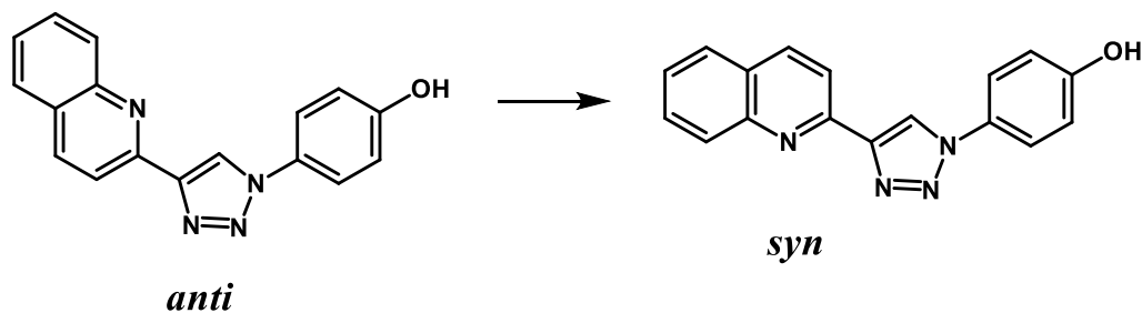
30 31 32 33 34 35 36 37 Scheme 1. Two different conformations of MIF180.
