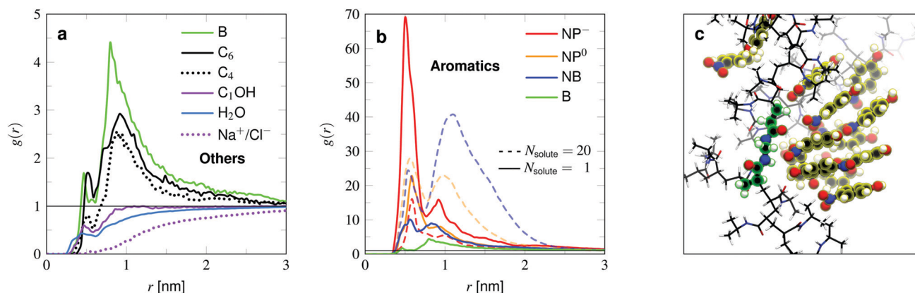
Fig. 4 (a) Normalized radial density profiles of the solutes with respect to the COM of the BIS-linker for the low-adsorption species ( C_6 , C_4 , C_1\text{OH} , \text{Na}^+ , \text{Cl}^- ), plus benzene (— B) and water (— \text{H}_2\text{O} ) profiles for comparison. Note that in the case of methanol (— C_1\text{OH} ) and sodium chloride (··· \text{Na}^+/\text{Cl}^- ) simulations were carried out with 30 molecules or 3 ion pairs, respectively. Panel (b) shows much stronger adsorbing molecules BZ, NB, \text{NP}^0 , \text{NP}^- , all of aromatic nature, in the high dilution limit (—) and more concentrated solutions with a total of 20 (---) molecules (and 20 \text{Na}^+ counterions in the case of \text{NP}^- ) per simulation. (c) Simulation snapshot showing a stacking of \text{NP}^0 in the cross-link region. BIS and \text{NP}^0 are highlighted green and yellow respectively, PNIPAM is shown in licorice representation. Note that the aggregation of the solutes usually looks less ordered than presented due to thermal fluctuations.
