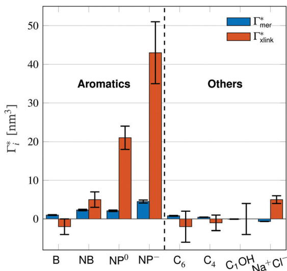
Fig. 5 Adsorption coefficients ( \Gamma^* = \Gamma/\rho_0 ) quantifying the binding affinities of different solutes to one PNIPAM monomer \Gamma_{mer}^* and the cross-linker \Gamma_{xlink}^* in the infinite dilution regime, as summarized in Table 1. The adsorption to the monomers increases with size, e.g., compare C_4 \rightarrow C_6 . The aromatic molecules show the highest adsorption, which is magnified by increasing polarity B \rightarrow NB \rightarrow NP^0 \rightarrow NP^- , coinciding with a cross-linker-enhanced binding affinity.
