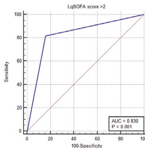
Figure 2. ROC curve evaluating the ability of LqSOFA >2 to predict mortality. Area under the curve (AUC)=0.830, P < 0.001 .
