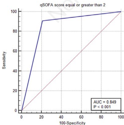
Figure 1. ROC curve evaluating the ability of qSOFA \geq 2 to predict mortality. Area under the curve (AUC)=0.849, P < 0.001 .
