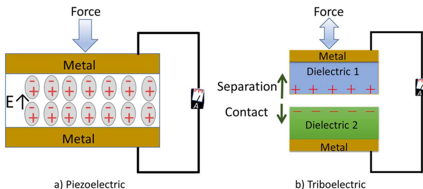
Figure 3. Schematics illustrating the sensing mechanisms of: a) Piezoelectric; b) Triboelectric.
