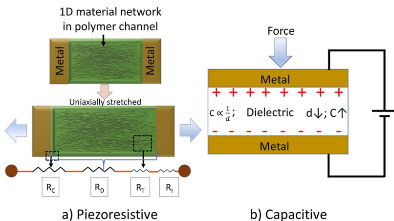
Figure 2. Schematics illustrating the sensing mechanisms of: a) Piezoresistive and b) Capacitive. R_C is contact resistance, R_D is device dimensional resistance, R_T is tunnelling resistance between two 1D material, and R_I is intrinsic resistance of the 1D material.
