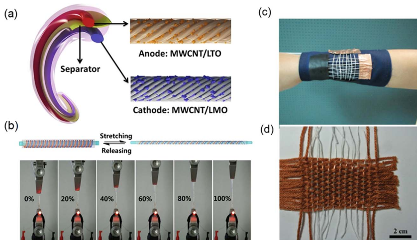
Figure 5. (a) Structure of the flexible wire-shaped lithium-ion battery composed of aligned woven yarns of active materials. (b) The wire-shaped battery can power a LED when stretched to double its length. (c, d) Fiber-shaped lithium-ion batteries directly woven into flexible textiles. Reproduced with permission from Wiley-VCH, 2014 181 and the American Chemical Society, 2014. 184
