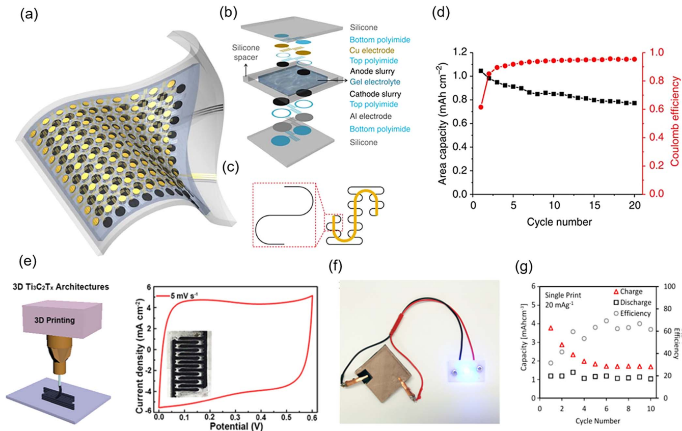
Figure 6. (a) Schematic of the island-bridge structure design for stretchable batteries with (b) an exploded-view layout of the various layers in the battery structure. (c) Illustration of “self-similar” serpentine geometries used for the interconnects (black: first-level serpentine; yellow: second-level serpentine) (d) Capacity vs cycling for the device. Reproduced with permission from Nature Publishing Group. 172 (e) 3D printing of MXene-type 2D material inks with suitable viscoelastic fingerprints layer by layer for current-collector-free electrodes. Reproduced with permission from Wiley-VCH, 2019. 186 (f) Single print PLA-based Li-ion battery powering an LED and (g) Capacity and Coulombic efficiency of the single print battery at a current density of 20 mA g -1 for 10 cycles. Reproduced with permission from American Chemical Society, 2013. 187
