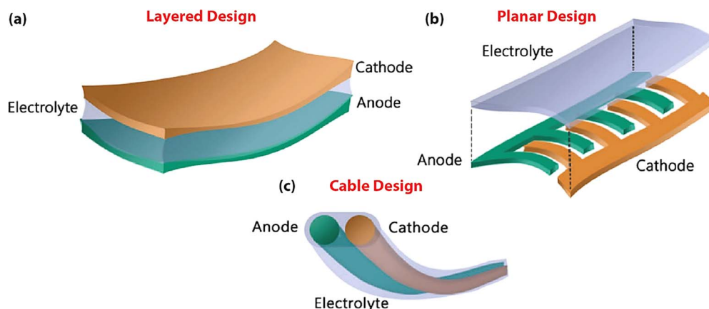
Figure 4. Schematics for three common designs for flexible energy storage systems. (Adapted from Ref. 162 with the permission of Royal society of Chemistry).
