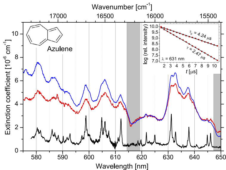
Fig. 4. Red trace: Broadband CRDS spectrum of azulene obtained from the ring-down time of light leaking from the cavity between 1.5 and 10.5 \mu\text{s} after plasma formation. The ring-down time was measured in steps of 0.5 \mu\text{s} accumulated over 500 plasma pulses (integration time of 250 \mu\text{s} ) per step. Blue trace: IBBCEAS spectrum of azulene obtained by accumulating the cavity output for 500 plasma pulses from 1.5 to 10.5 \mu\text{s} after plasma formation (gated data acquisition); total integration time of 4.5 ms. Determination of the extinction coefficient is based on the effective reflectivity shown in Fig. 3. Black trace: Arbitrarily scaled cavity ring-down absorption spectrum of jet-cooled azulene from [12] for comparison. Inset: Semi-logarithmic plot of the cavity output intensity showing the ring-down time measurements including the respective fit without and with azulene present in the cavity (red squares and dots respectively), measured at 631 nm (also compare Fig. 2).
