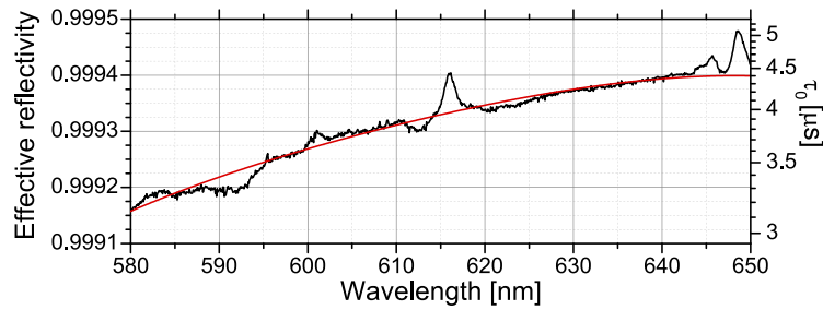
Fig. 3. Black trace: Effective mirror reflectivity (left-axis) calculated from the wavelength-dependent ring-down time of light leaking from the cavity (right-axis). Red trace: Fourth-order polynomial fit to the measured reflectivity spectrum.
