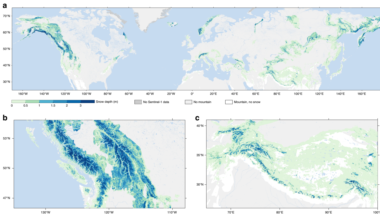
Fig. 4 Monthly snow depth retrieved by Sentinel-1. a Snow depth (m) over the Northern Hemisphere mountains. b Enlargement of a part of the western US and Canada. c As in panel b , but for a part of the Hindu-Kush Himalaya region. The -weekly 1 km 2 resolution Sentinel-1 retrievals are averaged over the month of February, 2018
