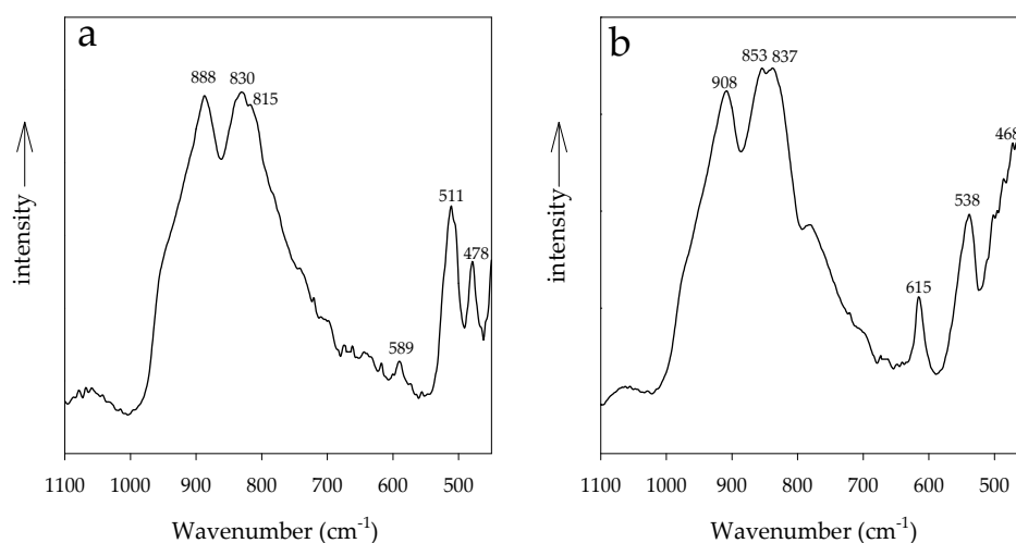
Figure 9. Infrared absorption spectra of samples 2 (a) and 3 (b).
