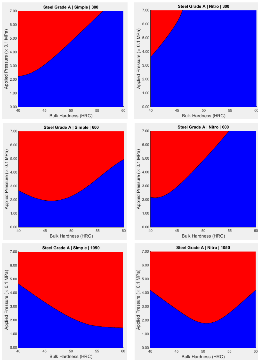
Figure 5. Maps of tribological performance for steel grade A, tested under three different rotational speeds 300, 600, and 1050 rpm: left column without surface treatment (before nitrocarburizing; right column after nitrocarburizing. The blue area corresponds to desirable uniform wear (Mode I), whilst the red one corresponds to non-desirable material behavior (Modes II, III, IV).
