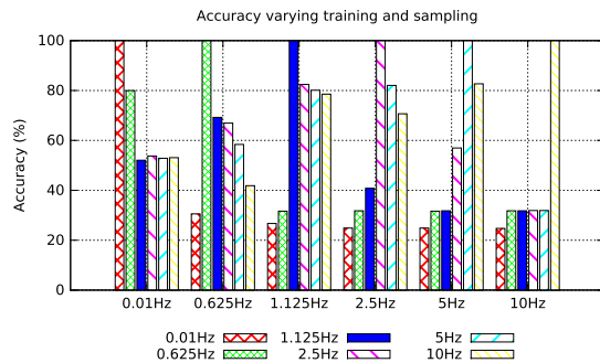
(b) Impact of r values on accuracy
