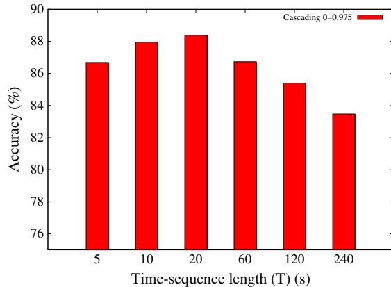
(a) Impact of T values on accuracy
