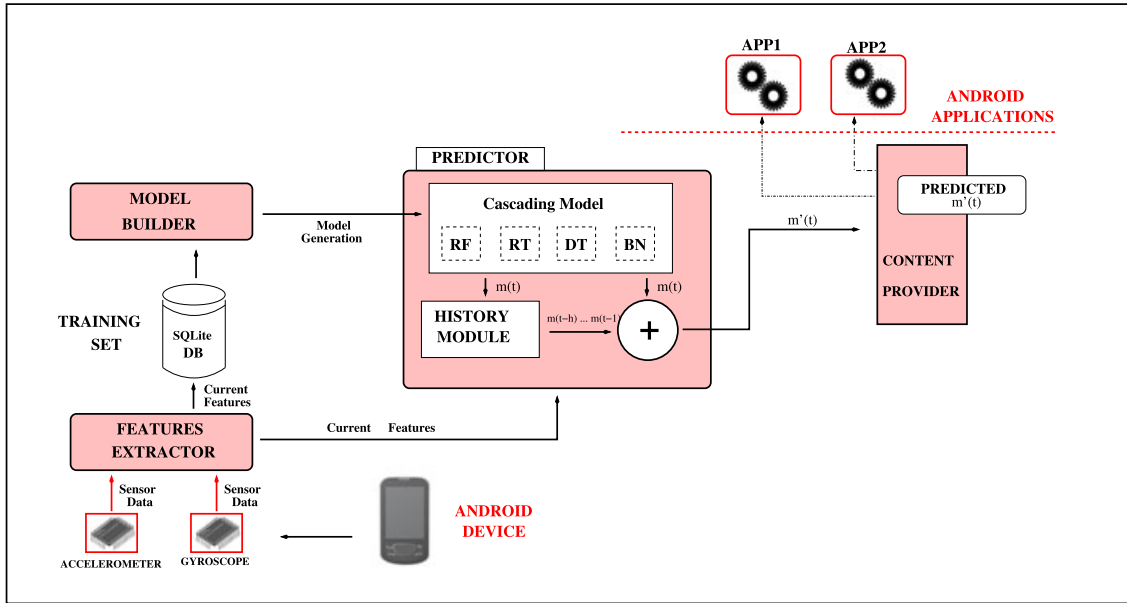
Figure 10. The What Am I Doing framework architecture. RF, Random Forest; RT, Random Tree; BN, Bayesian Network; DT, Decision Table.
