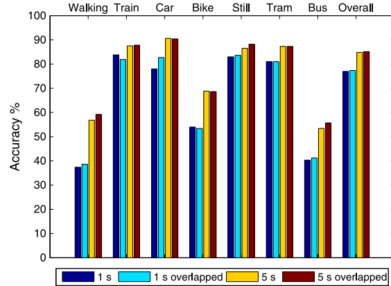
Figure 3. Comparison between overlapping and non-overlapping windows.
