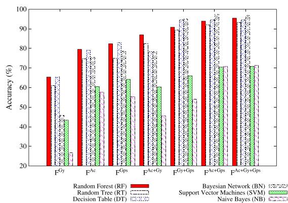
Figure 4. Average accuracy of learners on different combination of sensor data.
