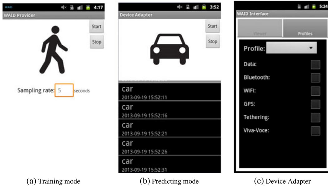
Figure 12. The screenshots of the What Am I Doing framework in Training Mode and Predicting Mode are shown in Figure 12(a) and (b), respectively. The Device Adapter interface is shown in Figure 12(c).
