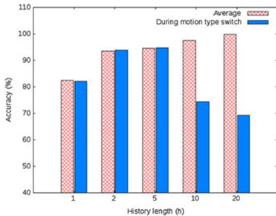
Figure 11. Impact of history length ( h ).
