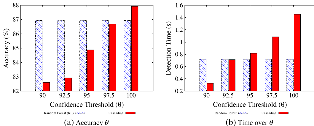
Figure 5. The accuracy of Algorithm 1 as a function of the confidence threshold \theta is shown in Figure 5(a). The average detection time of Algorithm 1 as a function of \theta is shown in Figure 5(b).
