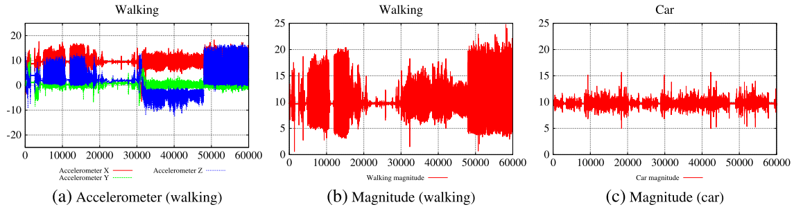
Figure 2. The raw accelerometer values (on the x , y , z axes) and the magnitude of the walking mode are shown in Figure 2(a) and (b), respectively. The magnitude of the car mode is shown in Figure 2(c).
