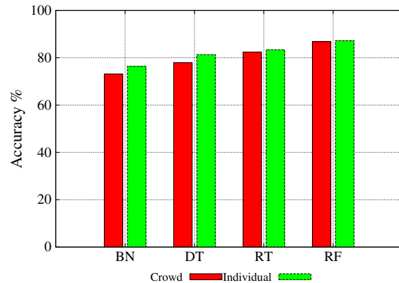
Figure 7. Data acquisition approaches: Individual versus Mobile-crowdsourcing.
