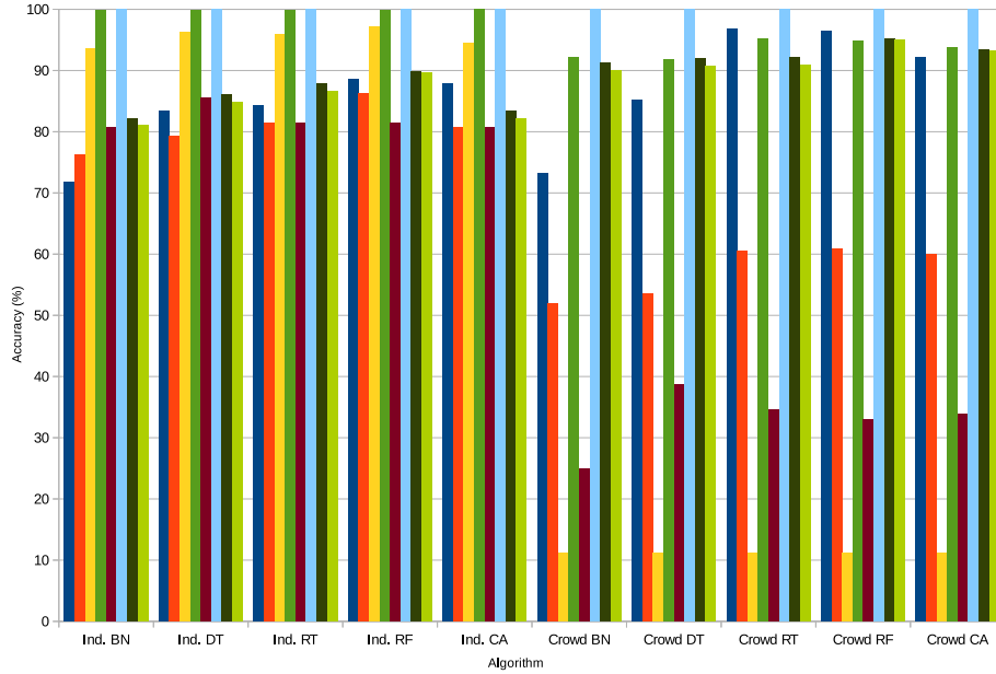
Figure 8. Data acquisition approaches: Individual versus Mobile-crowdsourcing per single user.
