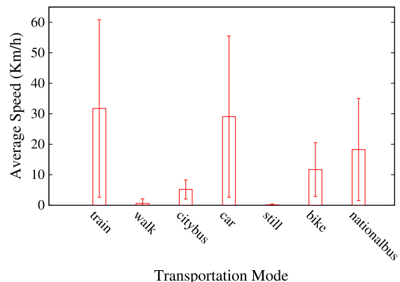
Figure 1. Average speed of different transportation modes.
