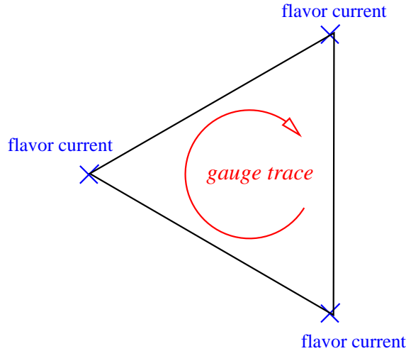
FIG. 2 (color online). The WZNW term is responsible for anomaly matching between the ultraviolet (microscopic) theory and the low-energy effective Lagrangian (macroscopic description). The anomalies in question are given by triangle graphs symbolically depicted in this figure, with flavor currents in the vertices—they are blind with respect to the gauge indices. The only information about the gauge structure comes from the trace in the loop.
