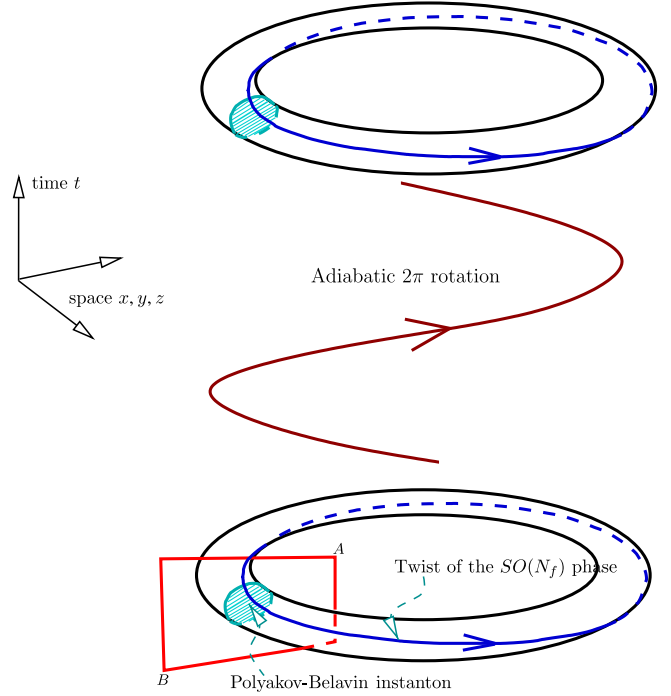
FIG. 3 (color online). Adiabatic rotation of a Hopf Skyrmion by the 2\pi angle. In the explicit calculation presented in this section, the toroidal object is rotated by 2\pi along an axis \hat{x}^3 which is perpendicular to the symmetry axis \hat{x}^2 . The contribution of the WZNW term to the action does not depend on the axis that we choose for the 2\pi rotation.
