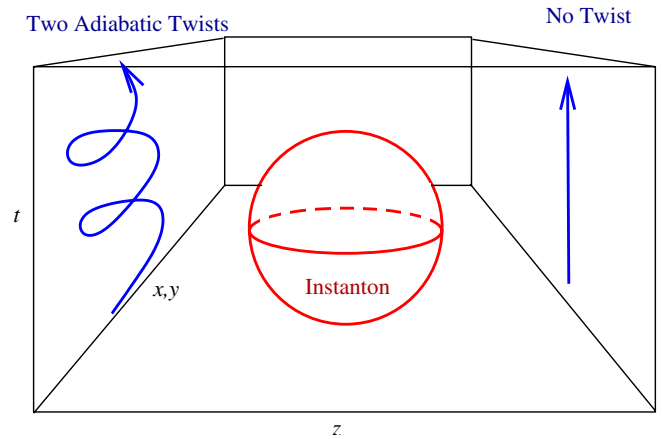
FIG. 1 (color online). The cube represents a four-dimensional space. The vertical coordinate is time t . We perform an adiabatic twist in t . The depth corresponds to the plane x, y where the vortex lies. The horizontal coordinate corresponds to z . On the left, in the space (x, y, t, z = -\infty) , we have a double-twisted vortex. On the right, at (x, y, t, z = +\infty) , we have a vortex with no twist. In the middle an instanton of \text{SO}(N_f) is generated. This explains why the integral over the Chern-Simons term gets continuously changed from 2 to 0 for N_f > 3 and from 4 to 0 for N_f = 3 .
