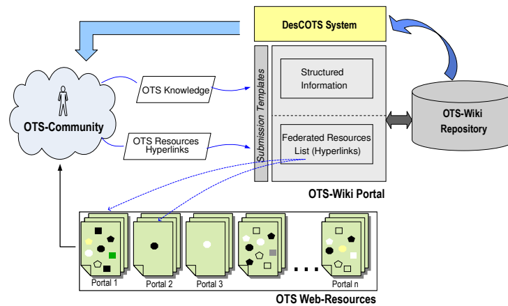
Fig. 1 OTS-Wiki Portal Main Interactions
