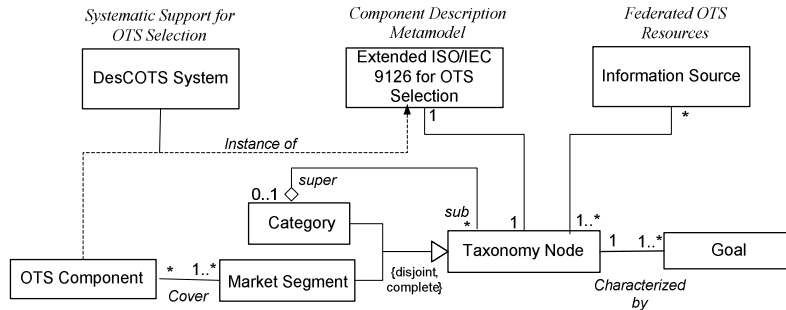
Fig. 2 Conceptual model for OTS-Wiki Portal Repository
