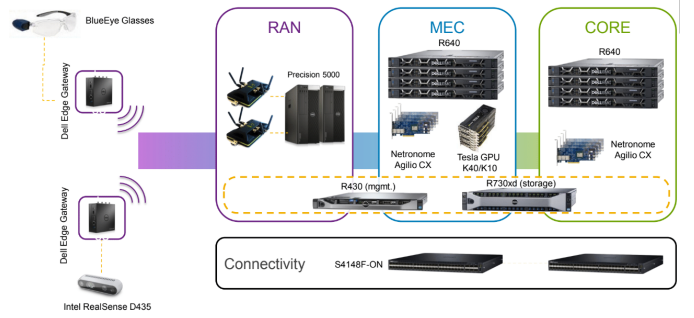
Fig. 7: 5G eHealth prototyping - hardware stack.
