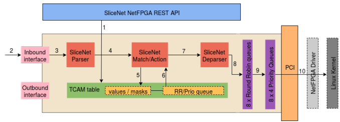
Fig. 4: SliceNet data plane traffic classification and QoS control architecture.
