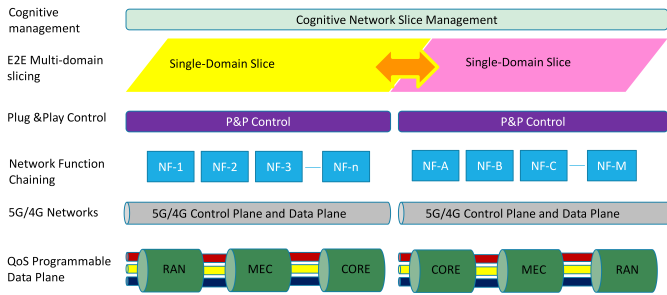
Fig. 1: Network slicing approaches in SliceNet.
