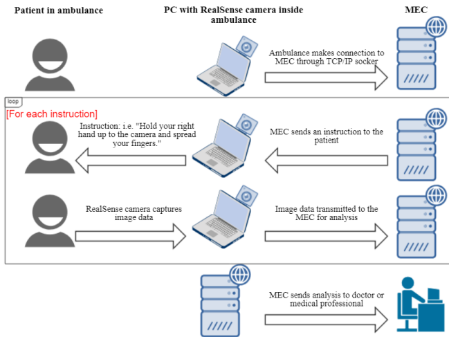
Fig. 2: High-level architecture for TeleStroke Assessment service.
