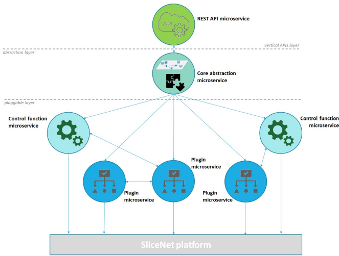
Fig. 6: P&P microservices architecture.
