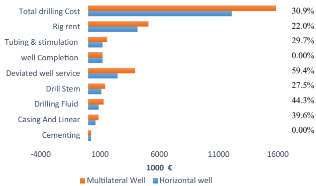
Fig. 11 Comparison of drilling and completion costs for fishbone well and single horizontal well
