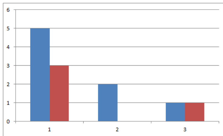
Figure5. 182: Topic Continuity: SATs v SETs
