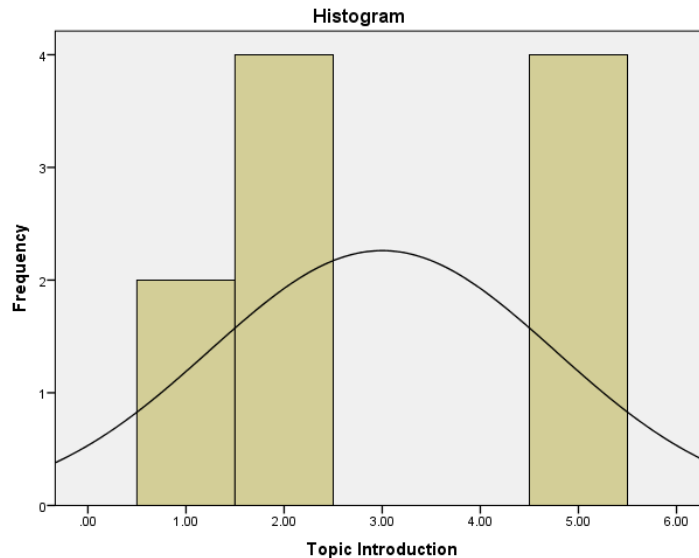
Figure5. 7: Topic signals employed for Topic Introduction in SATs
