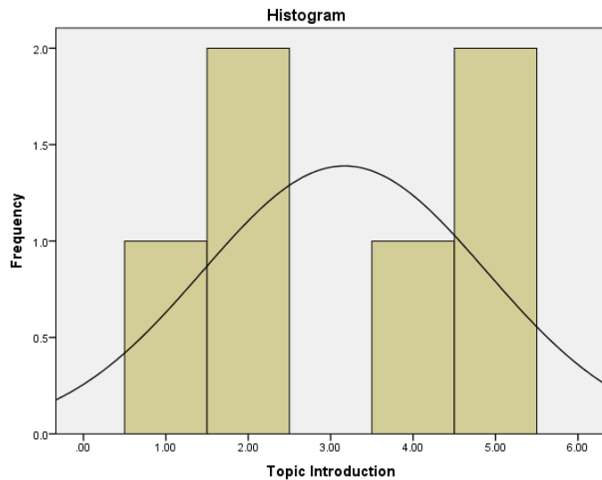
Figure5.11: Topic signals employed for Topic Introduction in SETs
