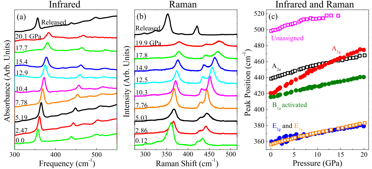
Figure 2: (a) Infrared and (b) Raman spectra of WS 2 nanotubes at the indicated pressures focusing on the observed vibrational modes. The number and position of modes are consistent with expectations, and the released spectra are taken after the compression cycle. (c) Frequency vs pressure for the infrared- (open squares) and Raman-active (closed circles) modes, displaying the stronger pressure sensitivity of the A 1g mode. The unassigned feature is likely a combination mode rather than a fundamental.
