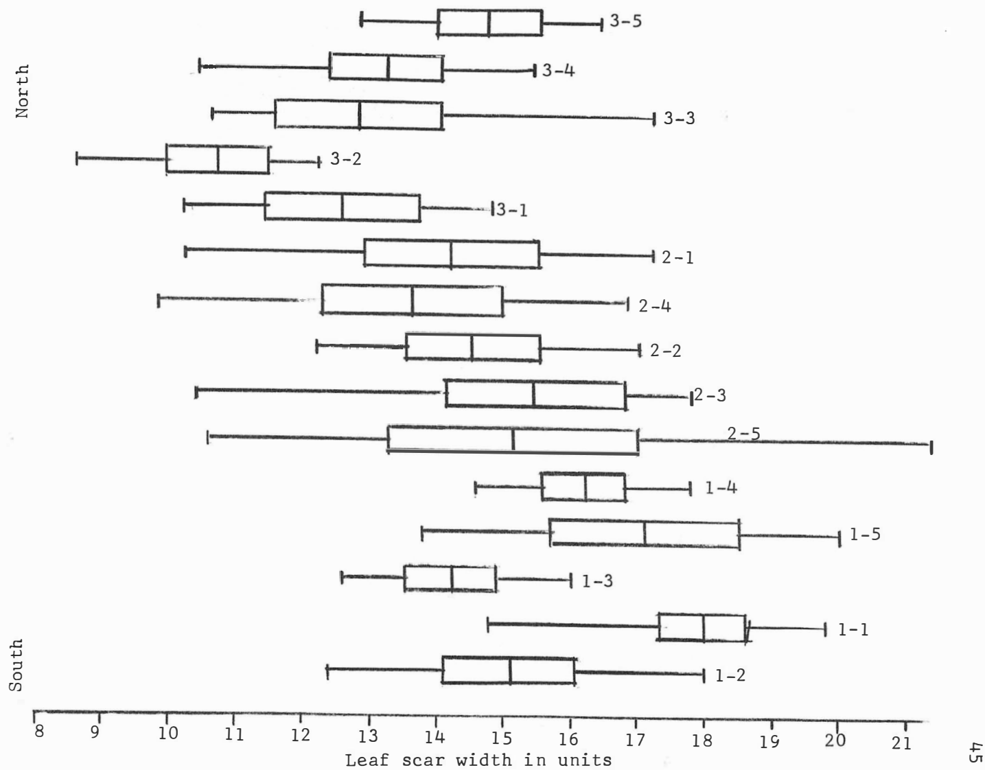
Figure 11. Leaf scar width in relative units, arranged by stands from north (up) to south (down).
