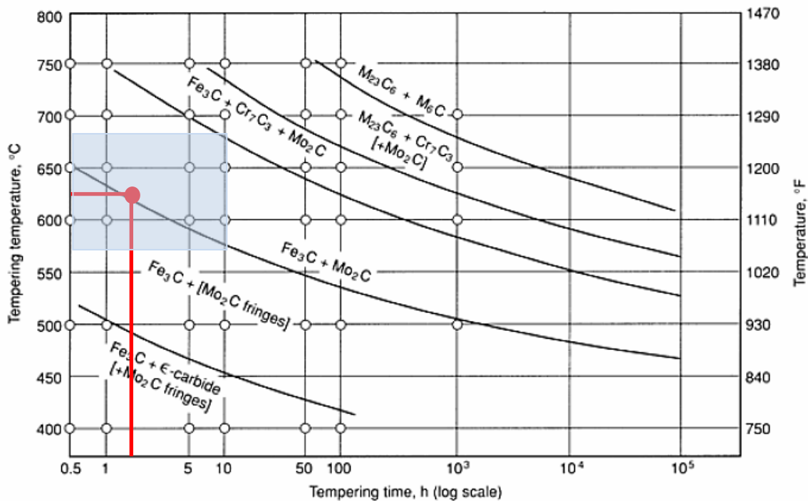
Figure 3. Baker and Nutting illustrate the sequence of carbide formation in Cr-Mo steel [49]. The blue box indicated the reheat cracking susceptible zone. Red lines show the approximate testing time (2 hrs) and temperatures (567-678°C (1050-1250°F)) of the Notched C-Ring Reheat Cracking Test.
